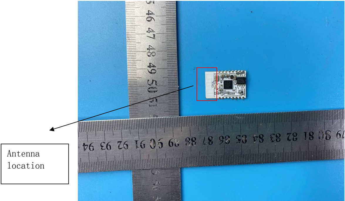
INTERNAL PHOTO OF SAMPLE PCB
