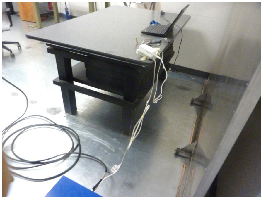
Figure 13 –Conducted Emissions Test Setup
