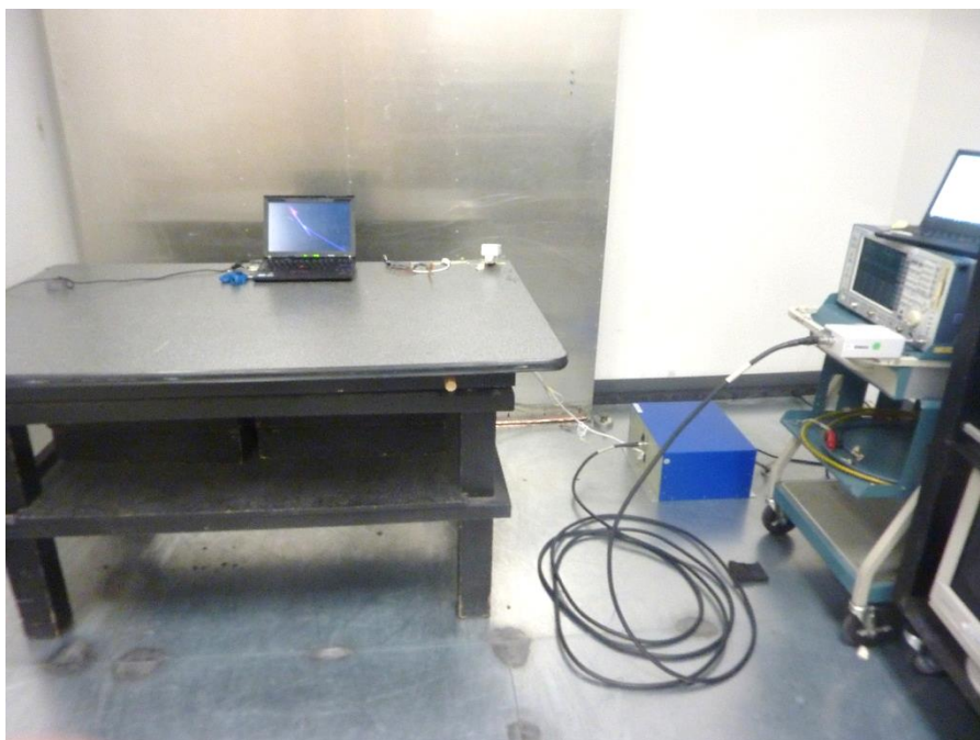
Figure 12 –Conducted Emissions Test Setup
