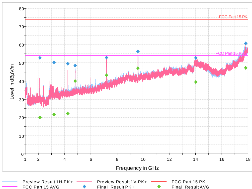
Plot 5. 1-18 GHz, 2402 MHz, 2Mbps
