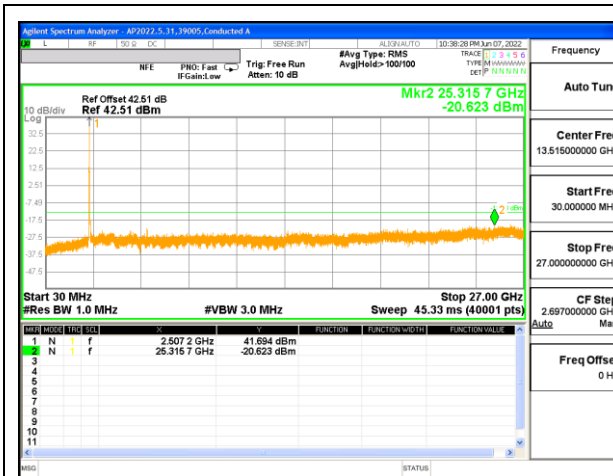
LTE B41 20MHz QPSK Low Channel
