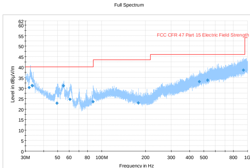
Figure 399 Radiated Emission 30MHz – 1GHz (5785 MHz) (20MHz Channel BW)
