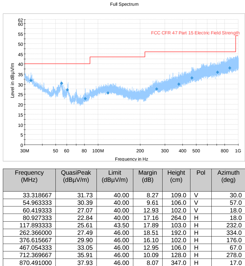
Figure 398 Radiated Emission 30MHz – 1GHz (5745MHz) (20MHz Channel BW)
