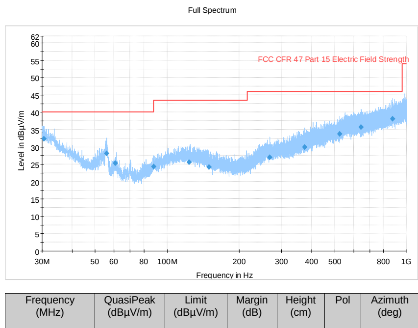
Figure 398 Radiated Emission 30MHz – 1GHz (5745MHz) (20MHz Channel BW)
