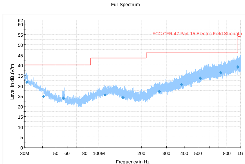
Figure 419 Radiated Emission 30MHz – 1GHz (5765/5785/5805MHz) (20MHz Channel BW)
