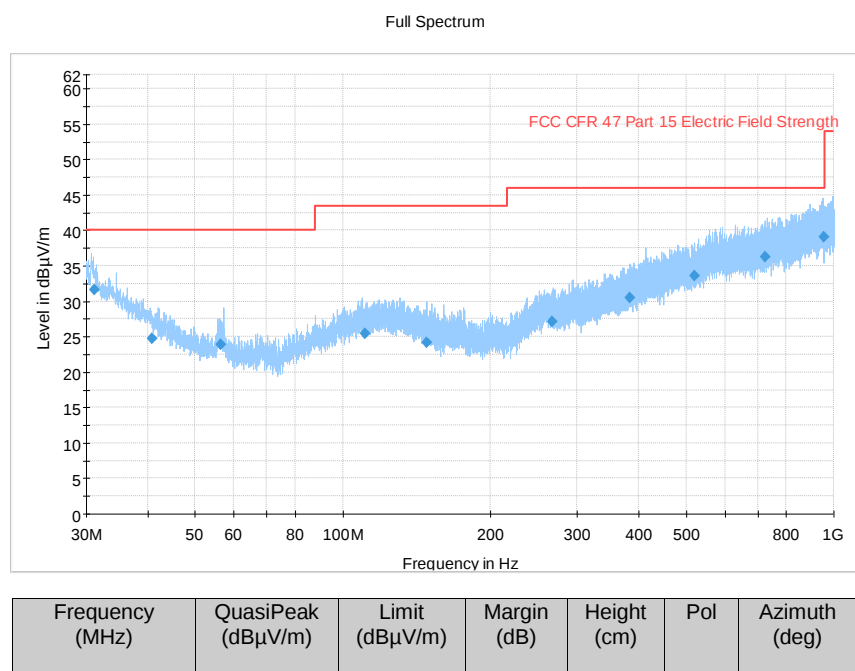
Figure 392 Radiated Emission 30MHz – 1GHz (5180/5200/5220MHz) (20MHz Channel BW)
