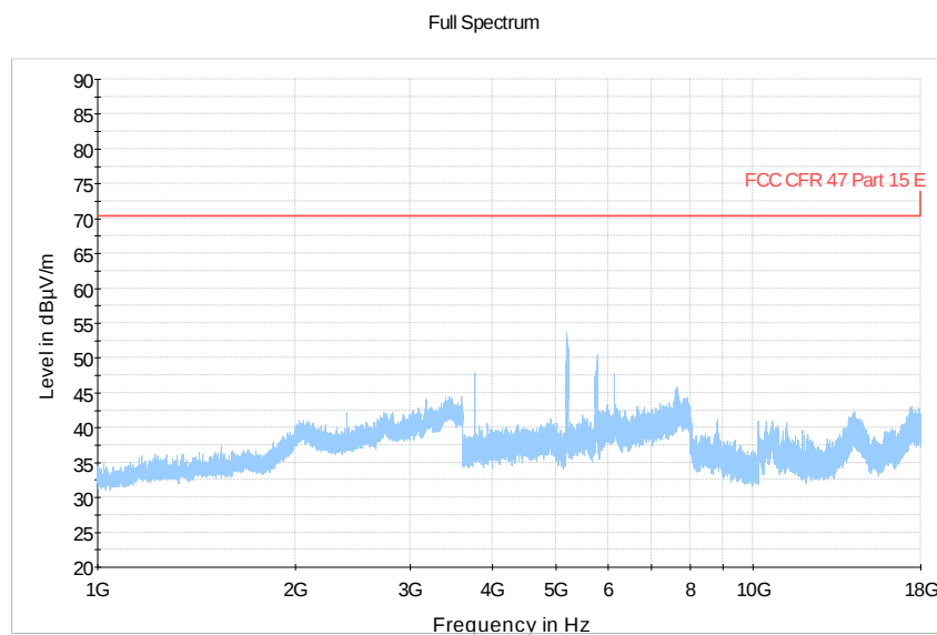
Figure 421 Radiated Emission 1GHz – 18GHz (5745/5765/5785MHz) (20MHz Channel BW)
