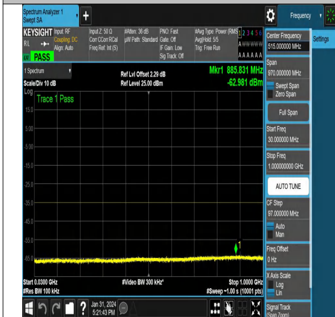
NTNV-N38-PC3-30-40-H-CP-QPSK-Edge_1RB_Left-Ant1-PAS
