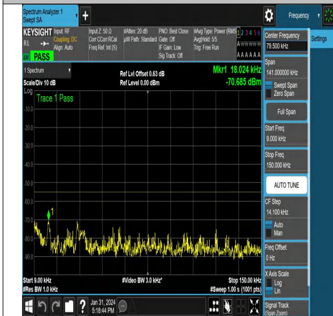
NTNV-N38-PC3-30-40-M-CP-QPSK-Edge_1RB_Right-Ant1-P
