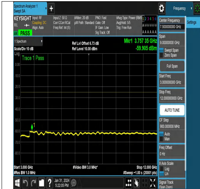
NTVN-N38-PC3-30-40-H-CP-QPSK-Edge_1RB_Left-Ant1-PAS
