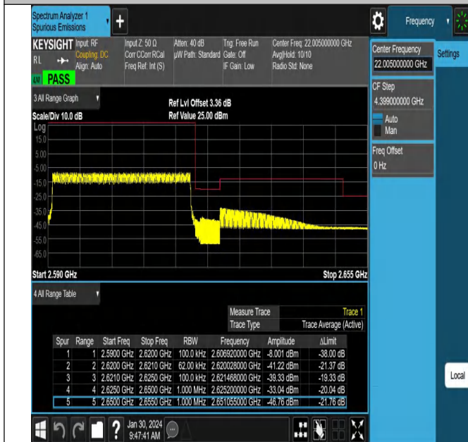
NTNV_N38_PC3_30_30_H_TID4_#1
