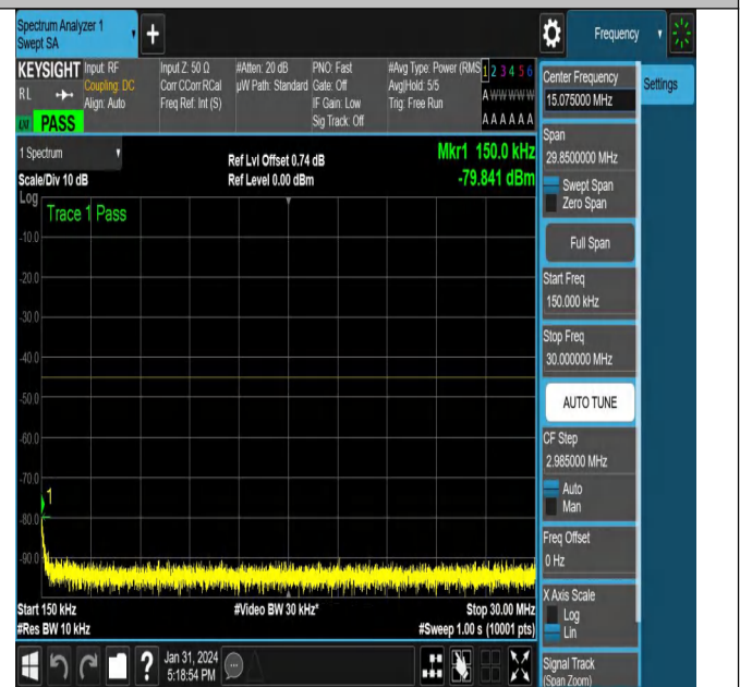
NTNV-N38-PC3-30-40-M-CP-QPSK-Edge_1RB_Right-Ant1-P
