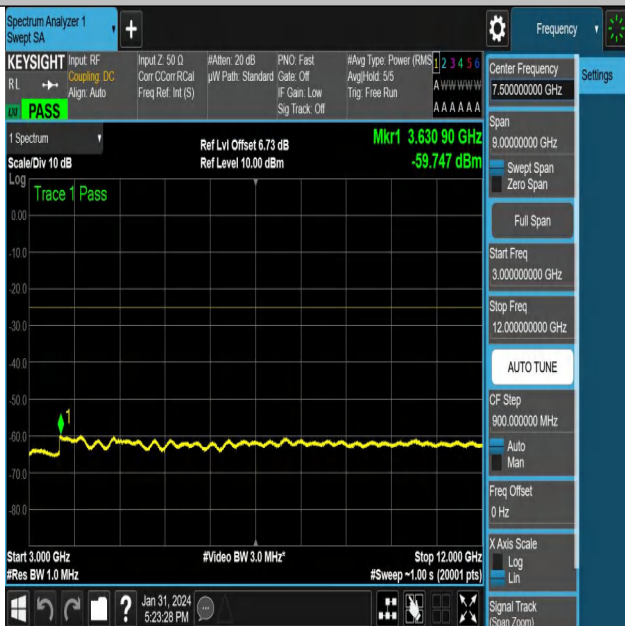
NTNV-N38-PC3-30-40-H-CP-QPSK-Edge_1RB_Right-Ant1-PA SS
