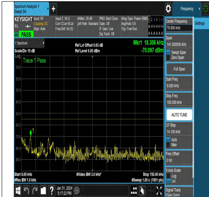
NTNV-N38-PC3-30-40-M-CP-QPSK-Edge_1RB_Left-Ant1-PA
