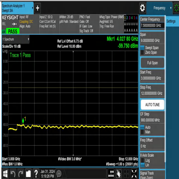
NTNV-N38-PC3-30-40-M-CP-QPSK-Edge_1RB_Right-Ant1-P ASS
