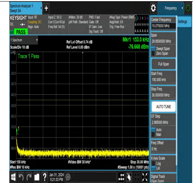
NTNV-N38-PC3-30-40-H-CP-QPSK-Edge_1RB_Left-Ant1-PAS
