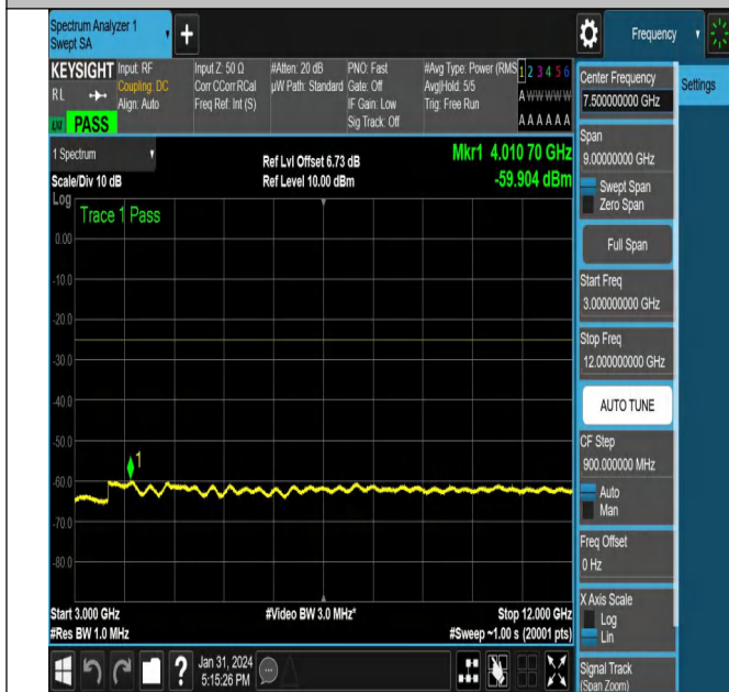
NTNV-N38-PC3-30-40-L-CP-QPSK-Edge_1RB_Right-Ant1-PA SS
