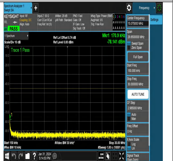
NTVN-N38-PC3-30-40-L-CP-QPSK-Edge_1RB_Right-Ant1-PA
