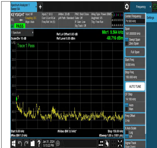
NTNV-N38-PC3-30-40-L-CP-QPSK-Edge_1RB_Left-Ant1-PAS S
