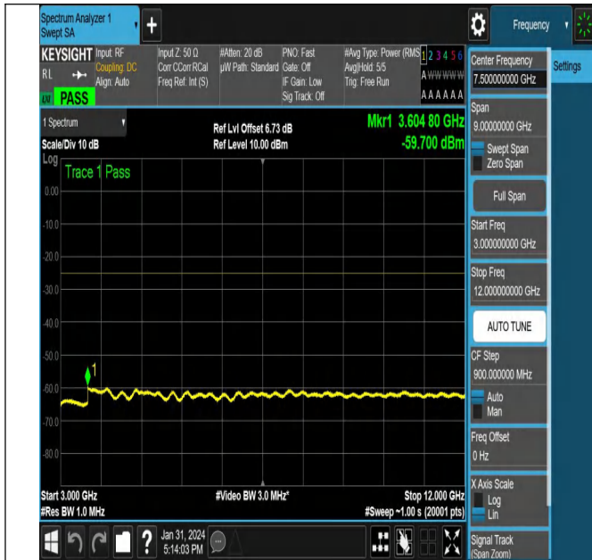
NTVN-N38-PC3-30-40-L-CP-QPSK-Edge_1RB_Left-Ant1-PAS
