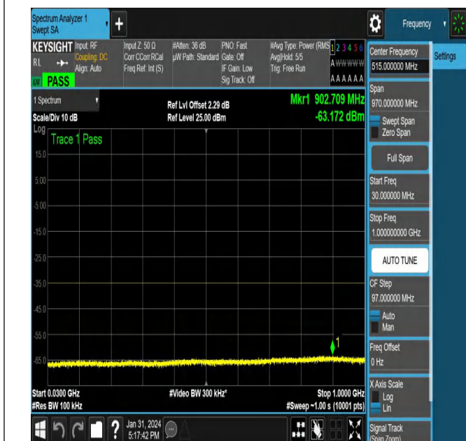
NTNV-N38-PC3-30-40-M-CP-QPSK-Edge_1RB_Left-Ant1-PA
