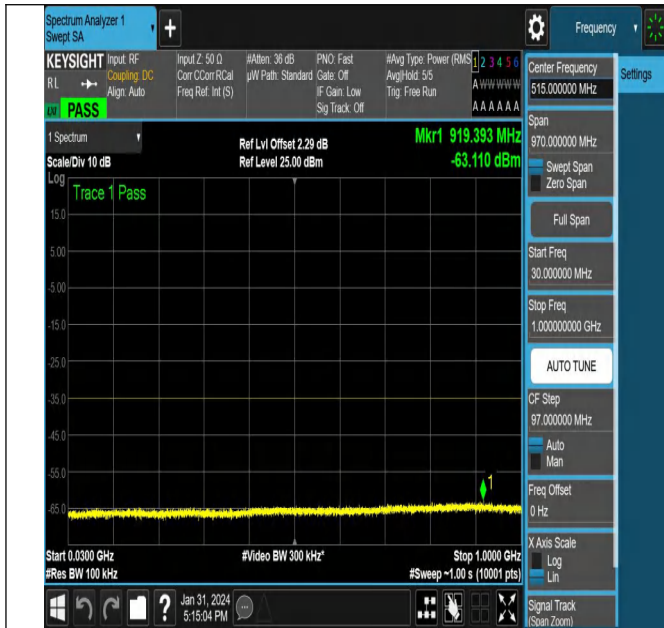
NTNV-N38-PC3-30-40-L-CP-QPSK-Edge_1RB_Right-Ant1-PA SS
