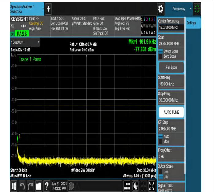
NTNV-N38-PC3-30-40-L-CP-QPSK-Edge_1RB_Left-Ant1-PAS S
