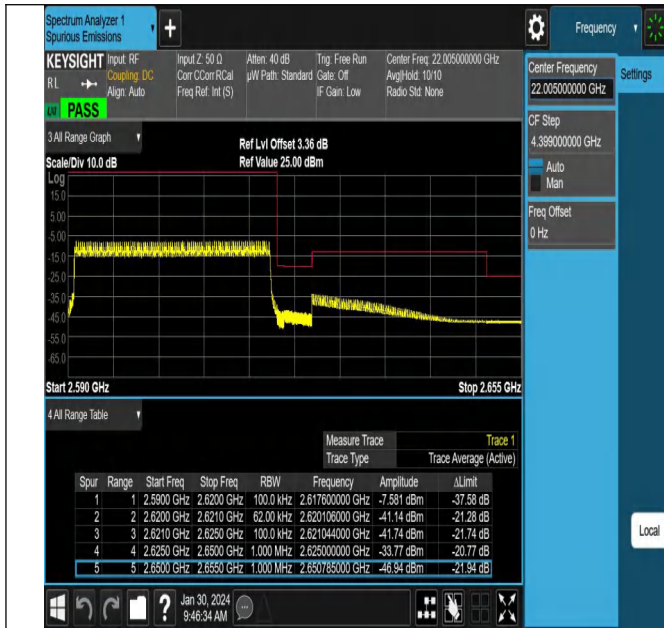
NTNV_N38_PC3_30_30_H_TID1_#1
