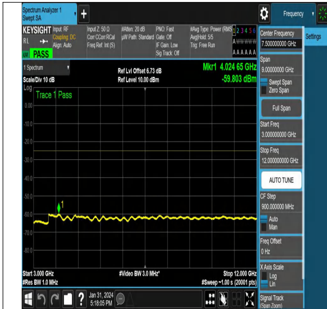
NTNV-N38-PC3-30-40-M-CP-QPSK-Edge_1RB_Left-Ant1-PA
