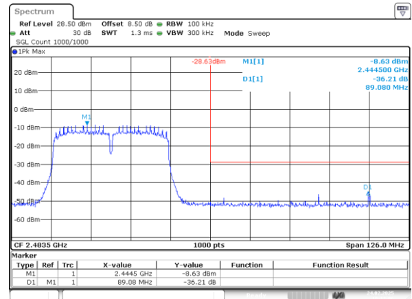
802.11n40_2452MHz_Chain 1
