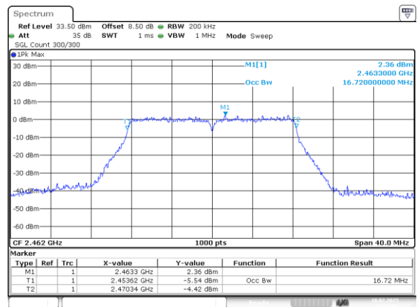
802.11g_2462MHz_Chain 1
