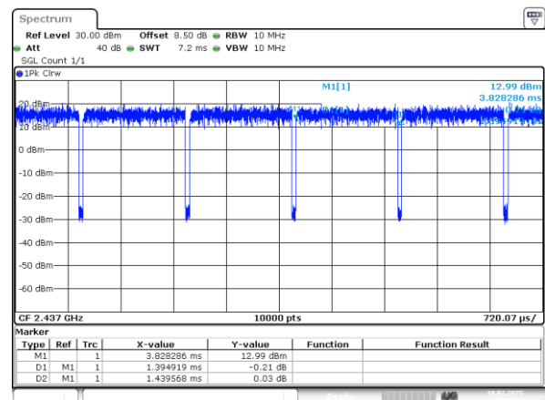
802.11g_2437MHz_Chain 1
