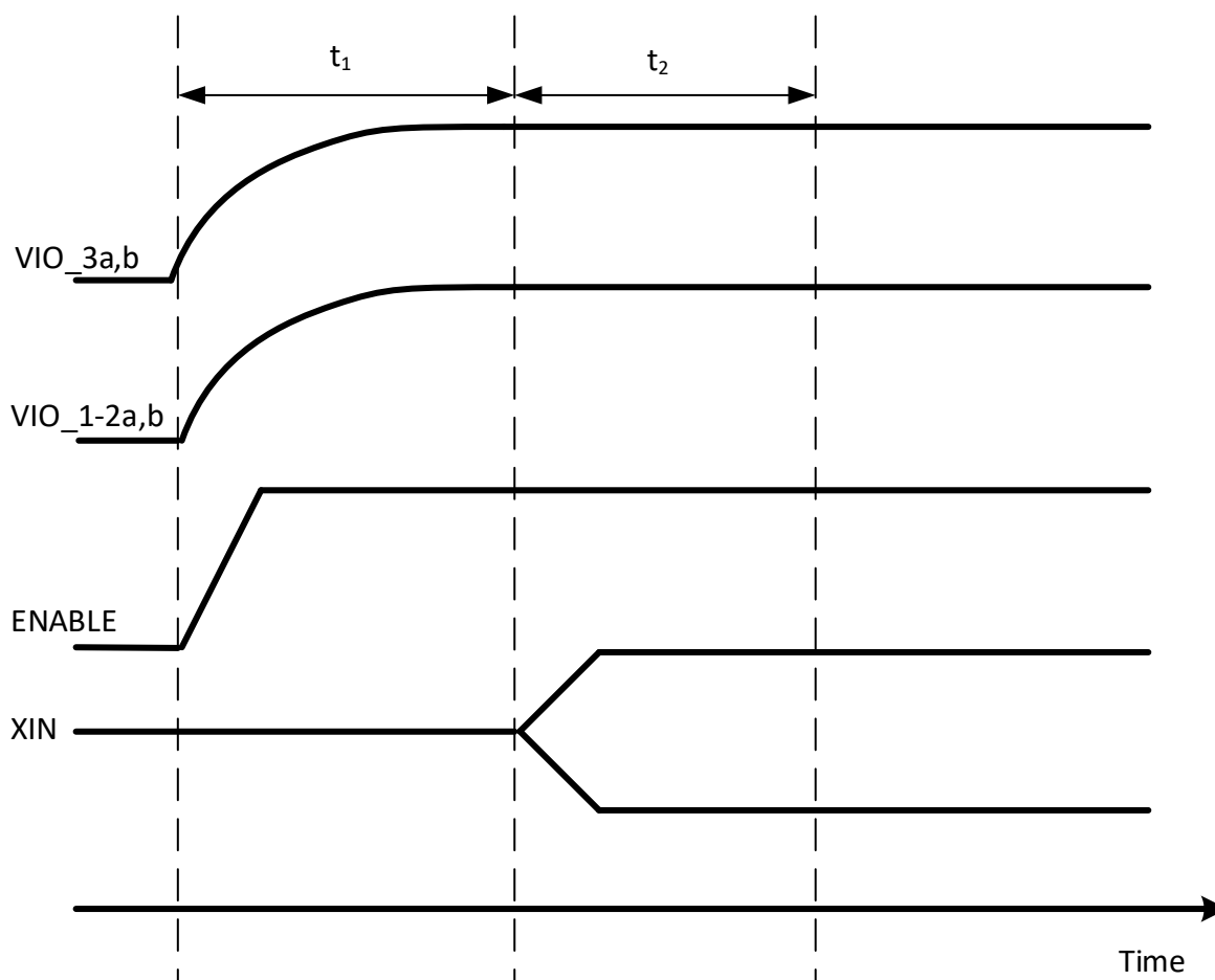
Figure 7.4. Power up sequence
