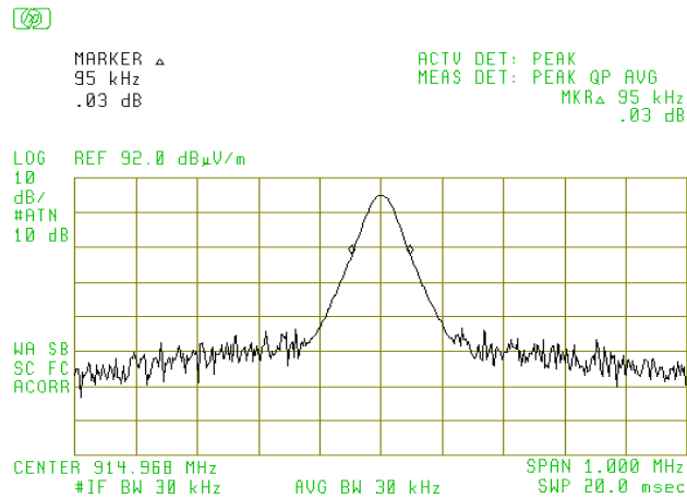
99% Bandwidth Plot
