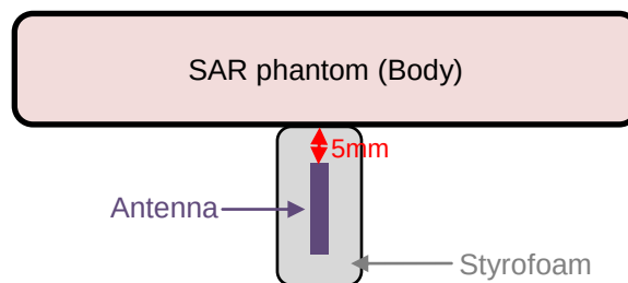
For antenna vertical position measurement
