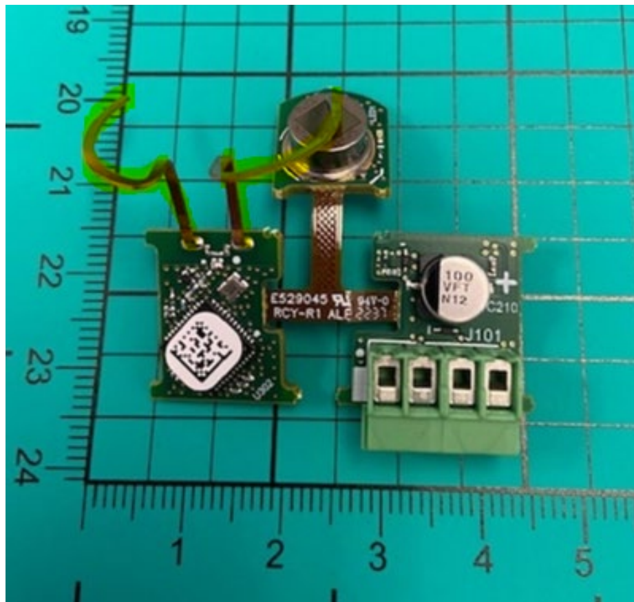
Internal Photo: (Antenna Highlighted)
