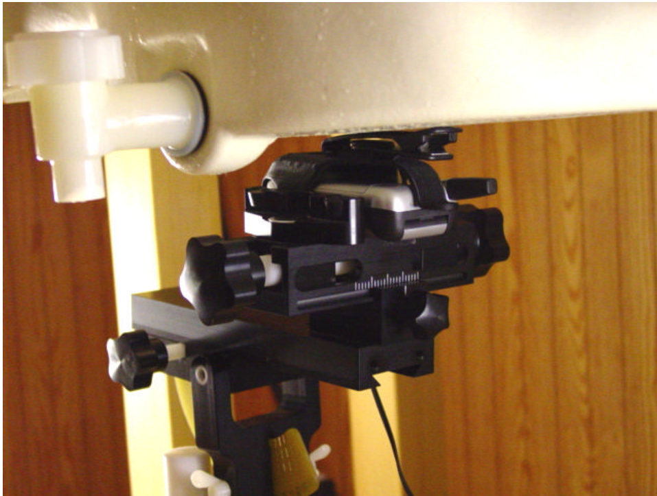
Figure 12.3 body SAR setup closed (with holster)
