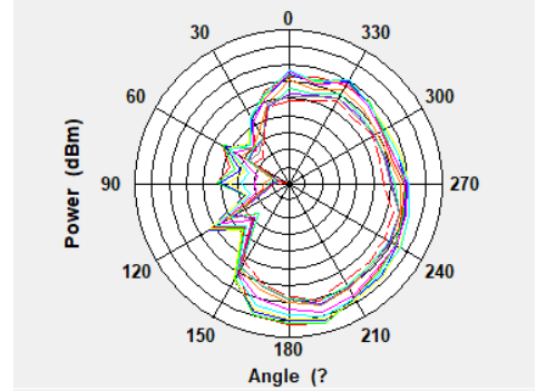
WBZ350 LGA_2D_YZ-Cut
