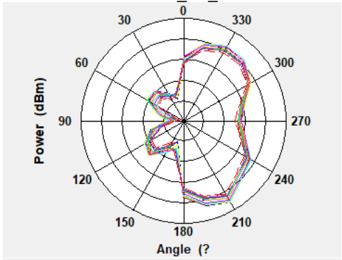
WBZ350 LGA_2D_YZ-Cut
