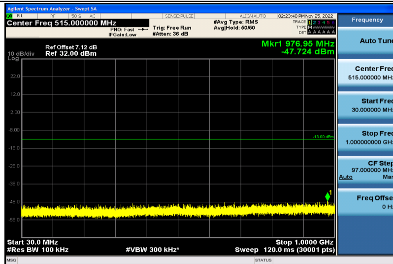
Band2-3MHz-64QAM-19185-1RB#0-30~1000MHz
