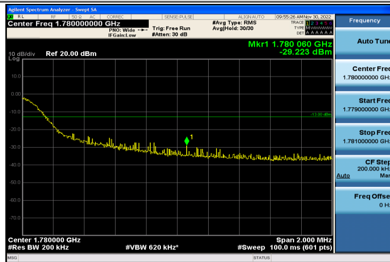
Band66-20MHz-64QAM-132572-100RB#0
