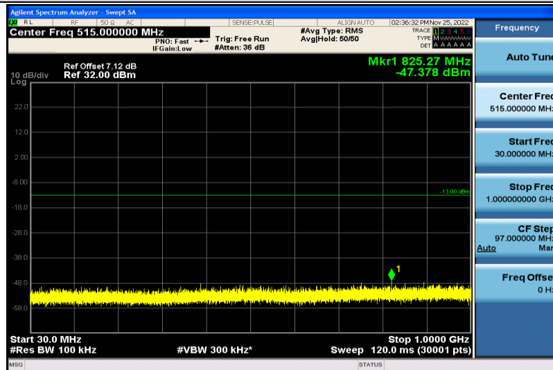
Band2-5MHz-64QAM-19175-1RB#0-30~1000MHz
