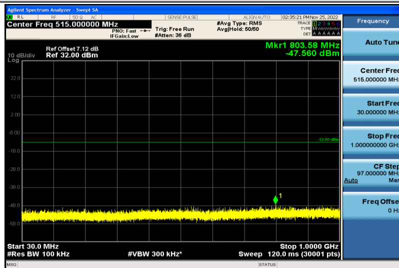
Band2-5MHz-64QAM-18625-1RB#0-30~1000MHz
