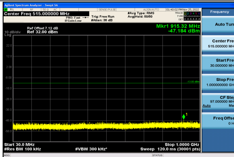
Band2-1.4MHz-64QAM-19193-1RB#0-30~1000MHz
