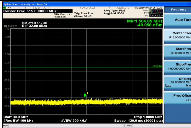
Band2-3MHz-64QAM-18900-1RB#0-30~1000MHz
