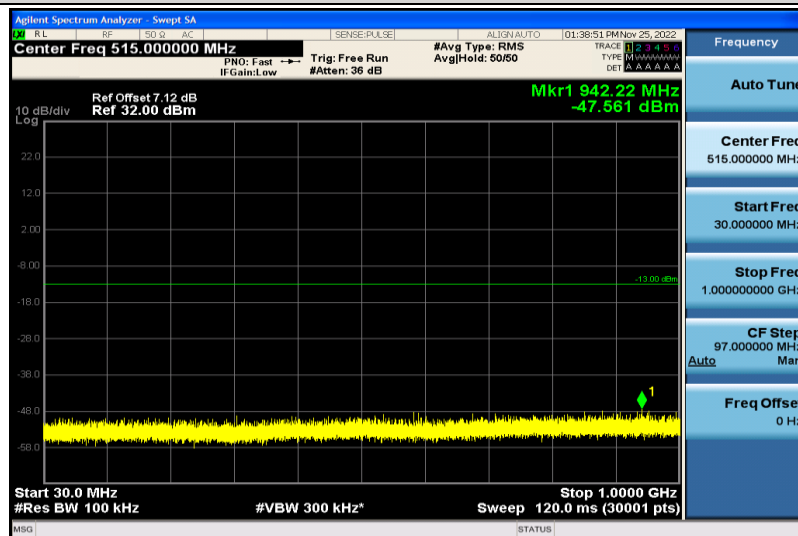
Band2-1.4MHz-64QAM-18607-1RB#0-30~1000MHz
