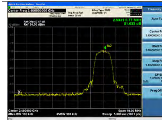
\pi/4 DQPSK(without hopping) Band Edge(CH.0)
