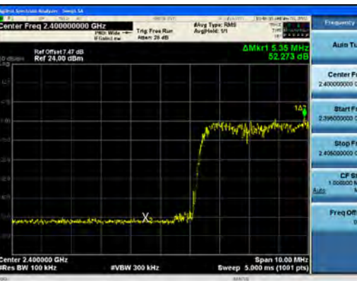
\pi/4 DQPSK(with hopping) Band Edge(CH.0)
