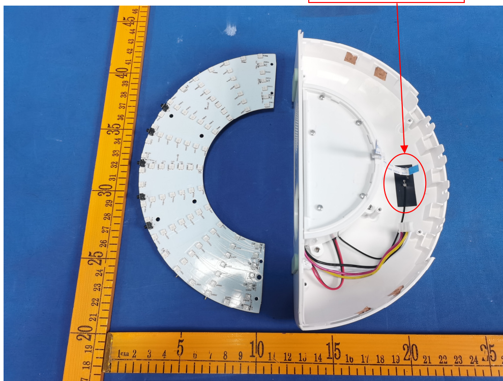
BT/BLE antenna
