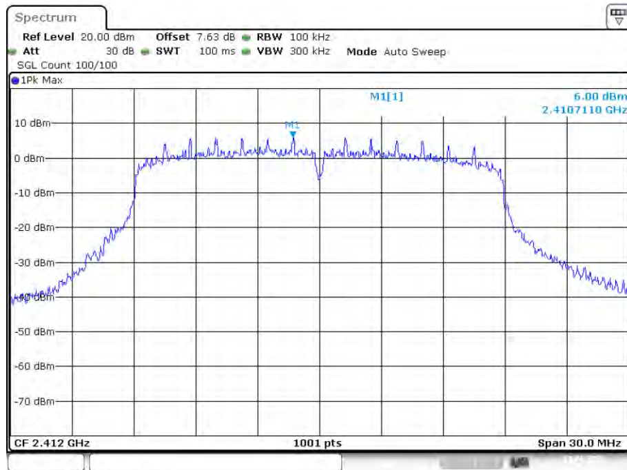
PSD NVNT n20 2412MHz Ant1+2
