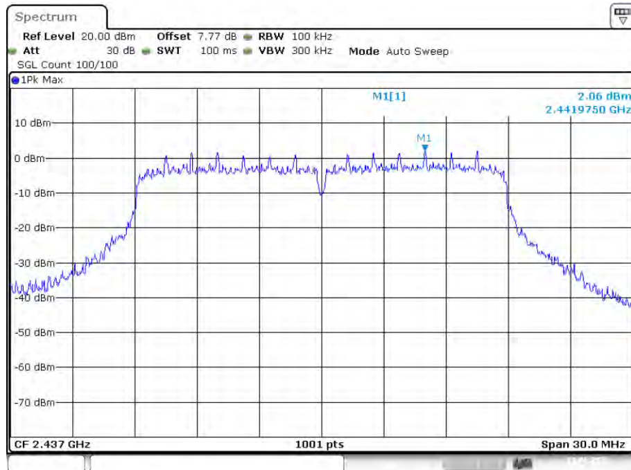
PSD NVNT n20 2437MHz Ant1+2
