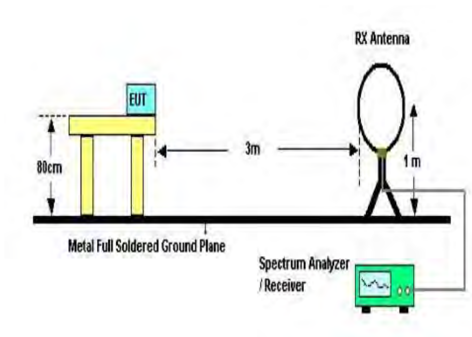
Below 30MHz Test Setup
