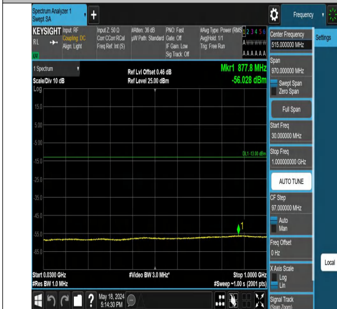
Band2-9400-30~1000MHz-PASS
