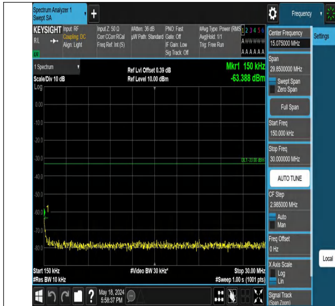
Band2-9538-1-0.15~30MHz-PASS
