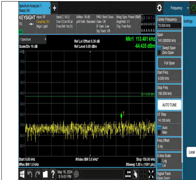
Band2-9538-0.009~0.15MHz-PASS
