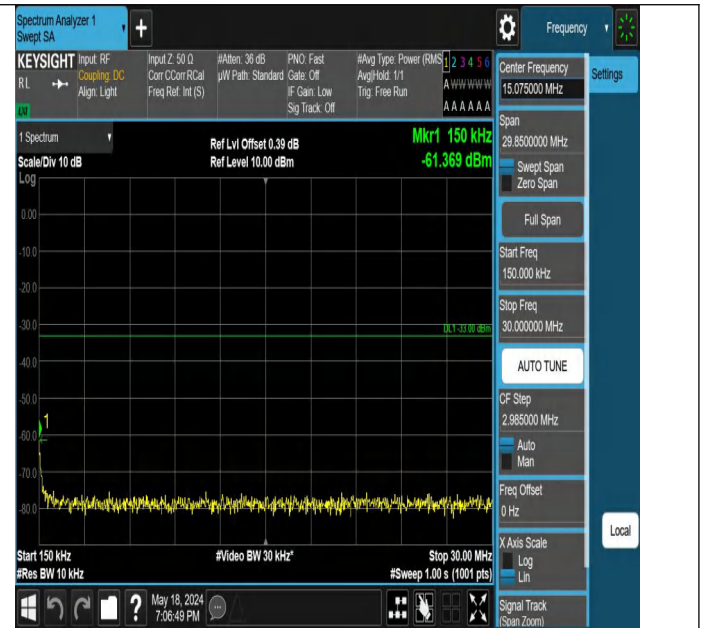
Band2-9262-1-0.15~30MHz-PASS
