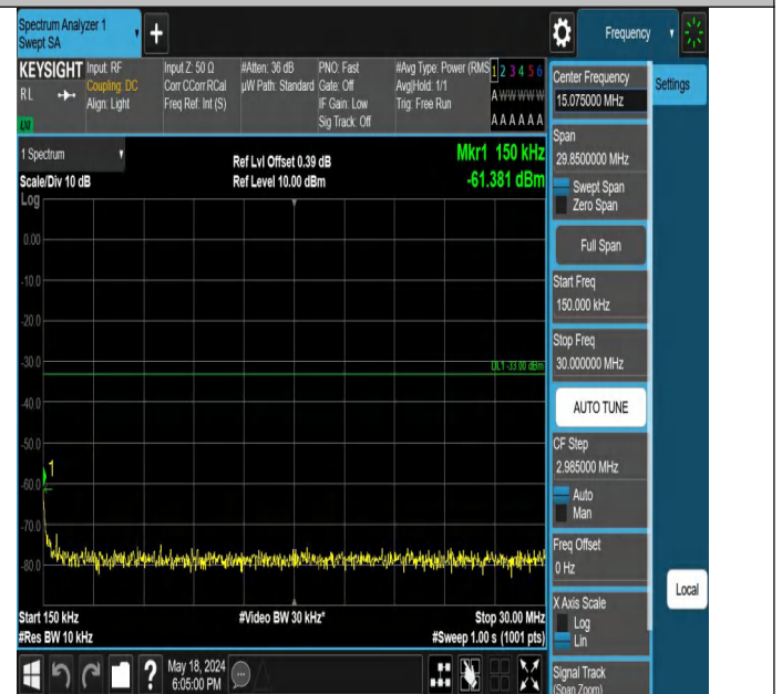
Band2-9538-4-0.15~30MHz-PASS
