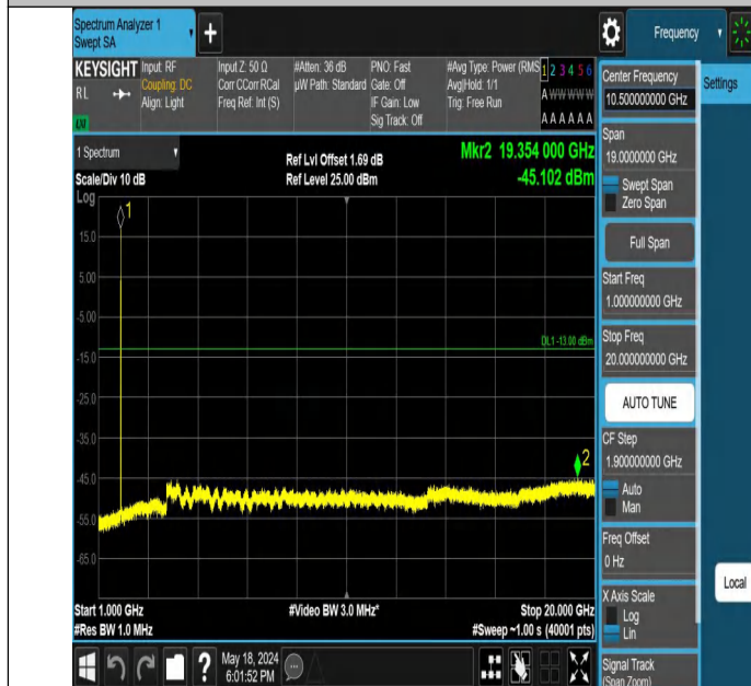
Band2-9262-3-1000~20000MHz-PASS
