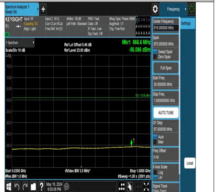
Band2-9538-4-30~1000MHz-PASS
