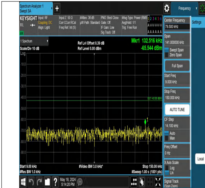
Band2-9400-0.009~0.15MHz-PASS
