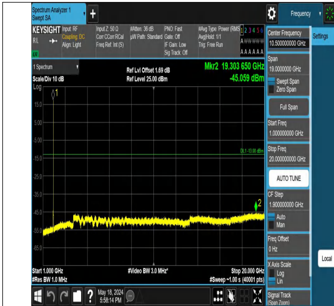
Band2-9400-1-1000~20000MHz-PASS
