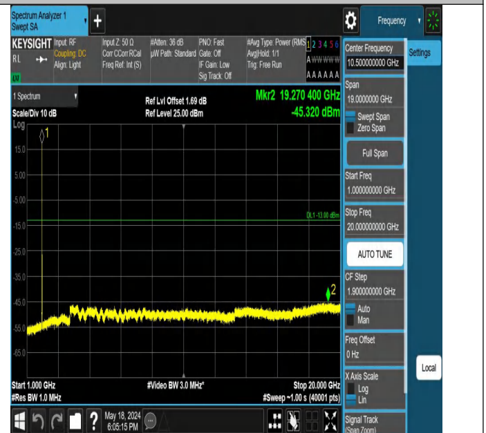
Band2-9538-4-1000~20000MHz-PASS
