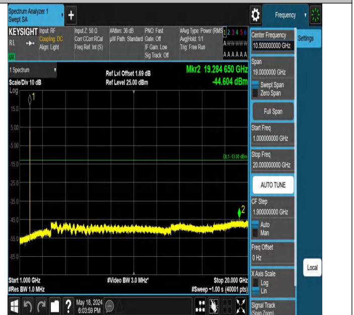
Band2-9262-4-1000~20000MHz-PASS
