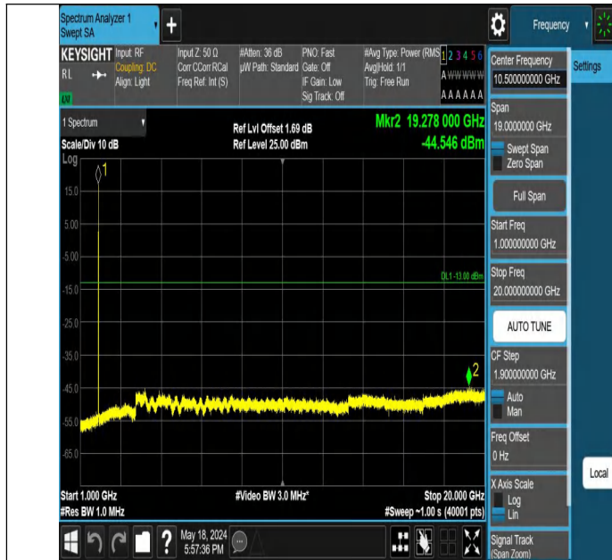
Band2-9262-1-1000~20000MHz-PASS
