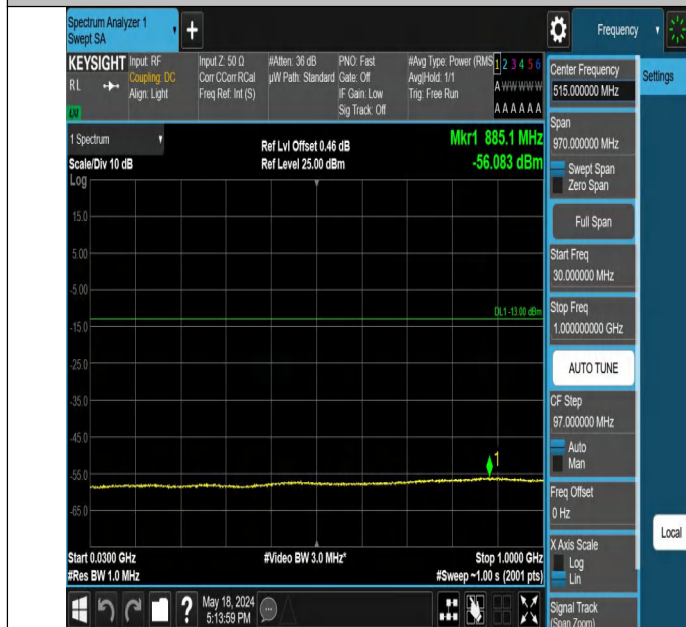
Band2-9262-30~1000MHz-PASS
