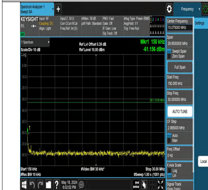
Band2-9538-3-0.15~30MHz-PASS
