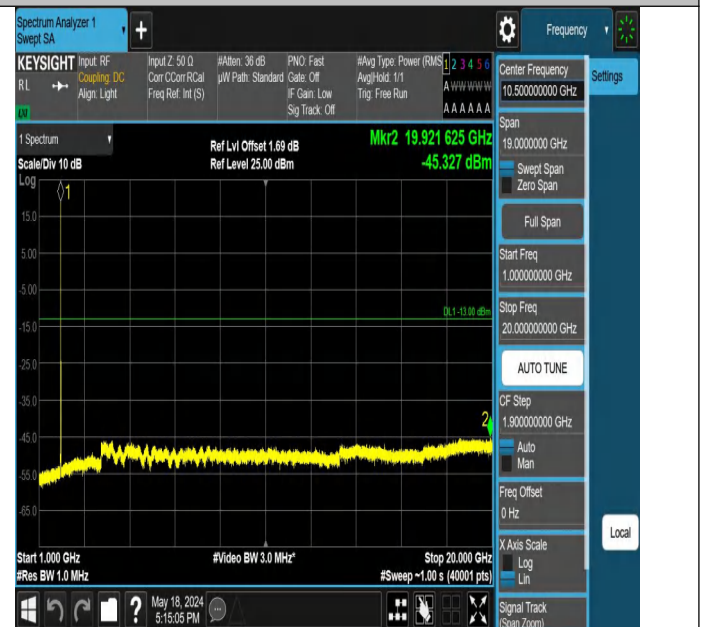
Band2-9538-1000~20000MHz-PASS
