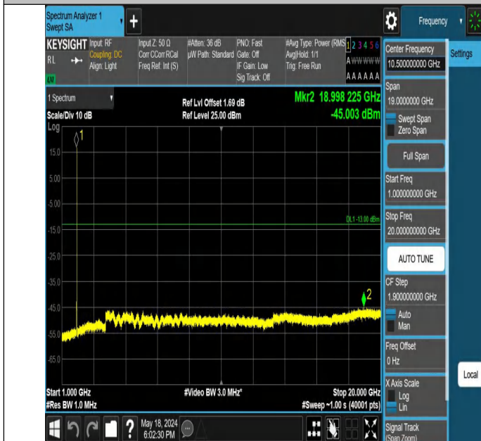
Band2-9400-3-1000~20000MHz-PASS
