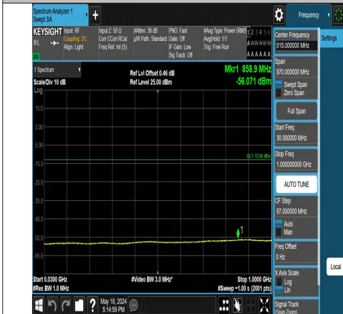
Band2-9538-30~1000MHz-PASS
