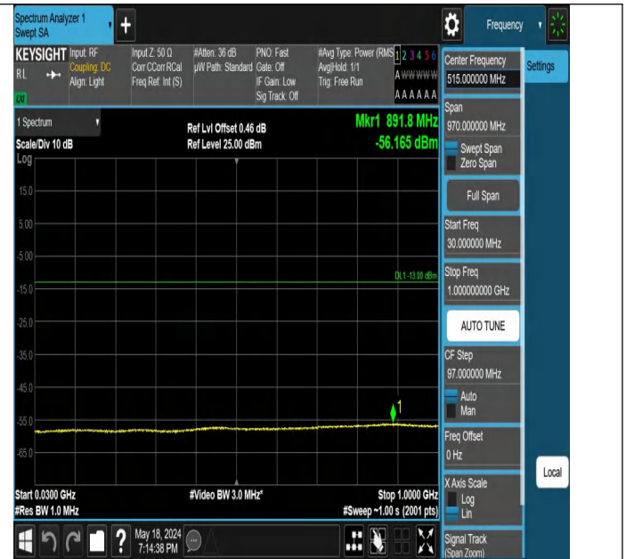
Band2-9262-4-30~1000MHz-PASS
