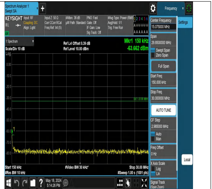
Band2-9400-0.15~30MHz-PASS
