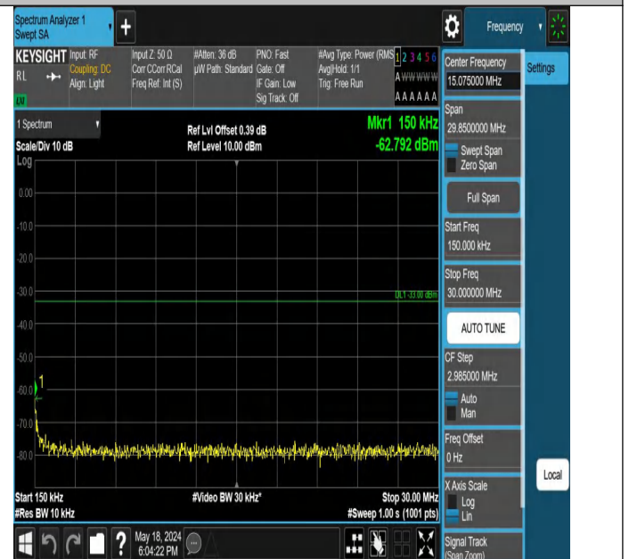
Band2-9400-4-0.15~30MHz-PASS
