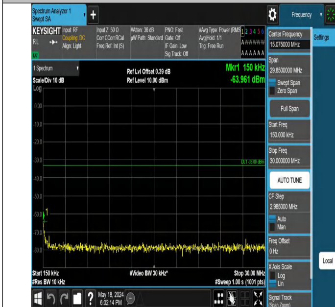
Band2-9400-3-0.15~30MHz-PASS
