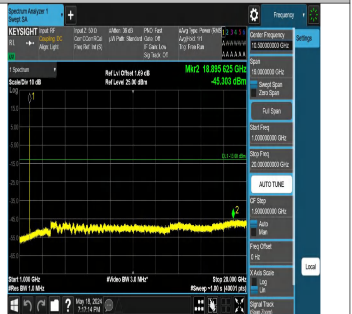
Band2-9262-5-1000~20000MHz-PASS
