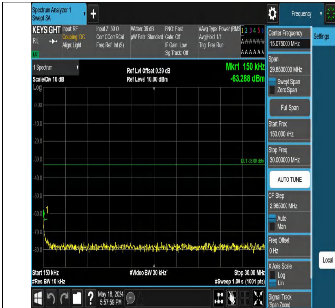
Band2-9400-1-0.15~30MHz-PASS
