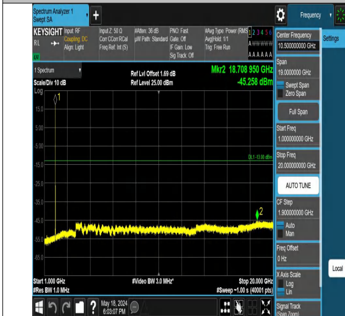
Band2-9538-3-1000~20000MHz-PASS
