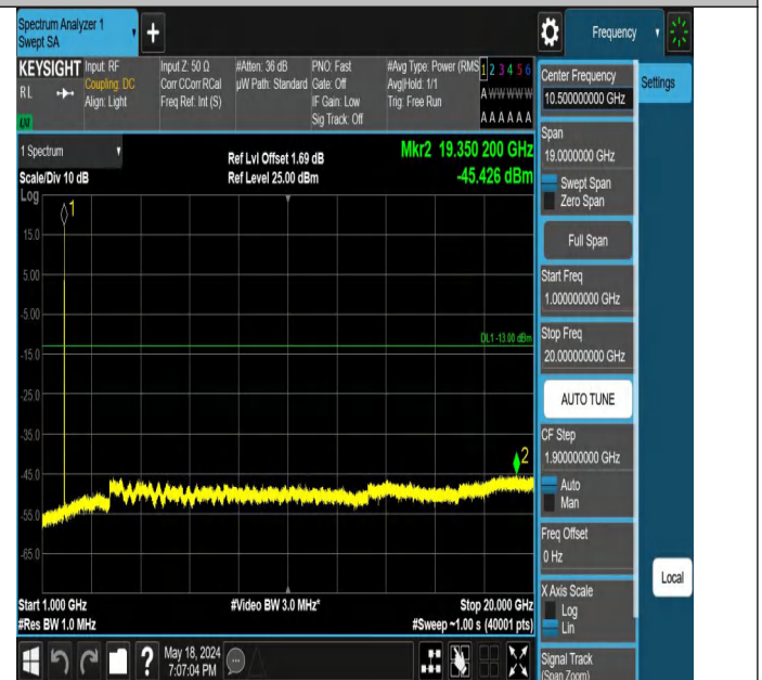
Band2-9262-1-1000~20000MHz-PASS
