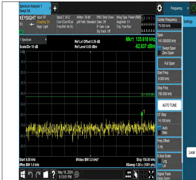
Band2-9262-0.009~0.15MHz-PASS
