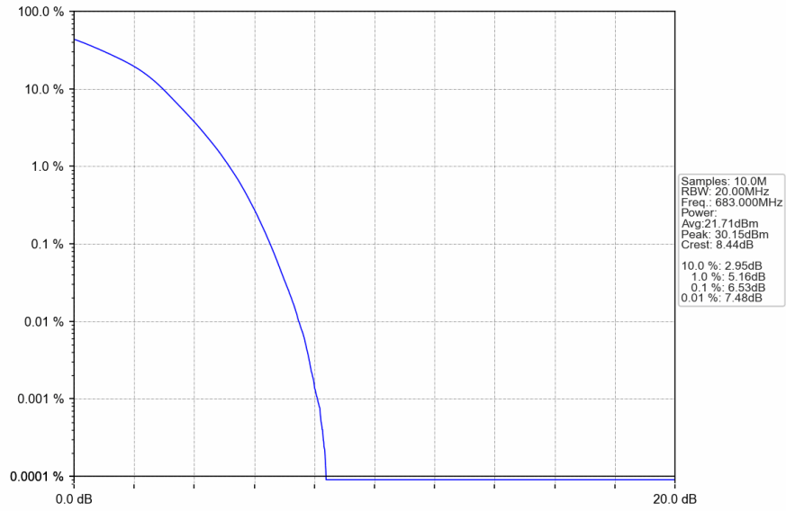
Band71_20MHz_16QAM_MCH_683MHz_RB_100_0_NTNV
