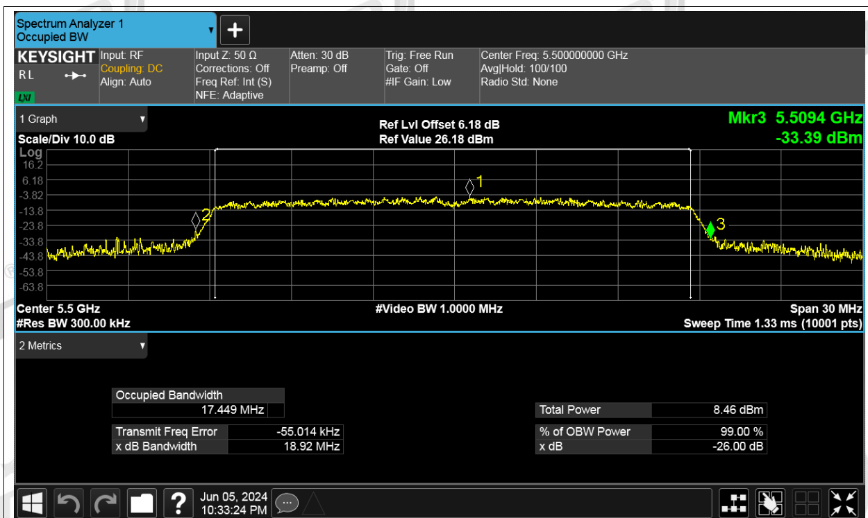
-26dB Bandwidth NVNT n20 5500MHz Ant3
