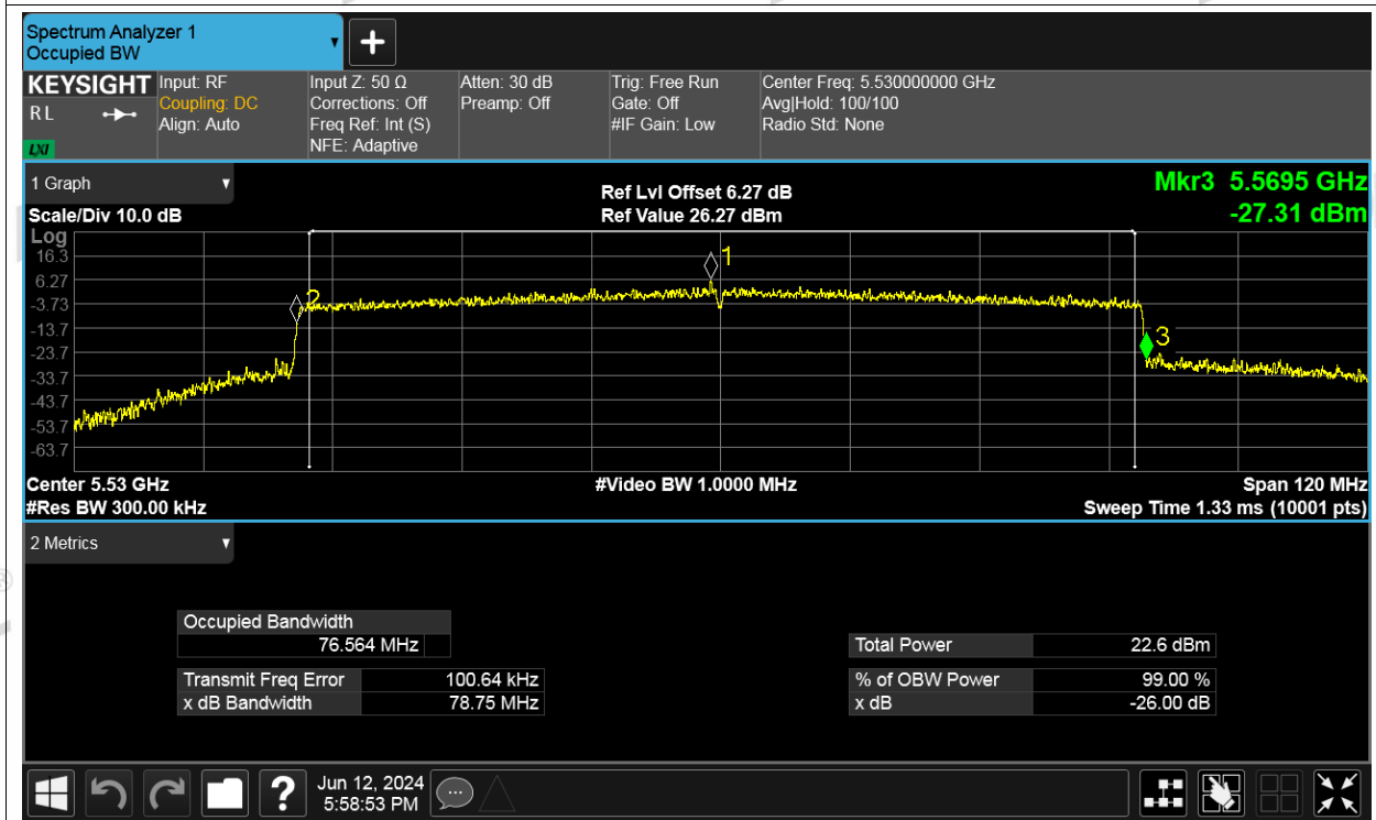
-26dB Bandwidth NVNT be80 5530MHz Ant2
