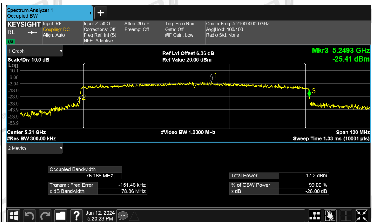
-26dB Bandwidth NVNT be80 5210MHz Ant3
