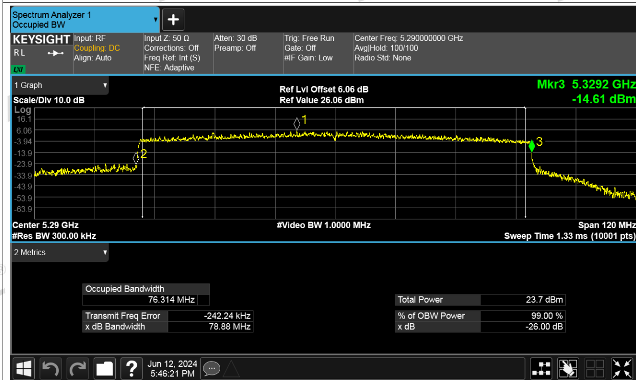
-26dB Bandwidth NVNT be80 5290MHz Ant3
