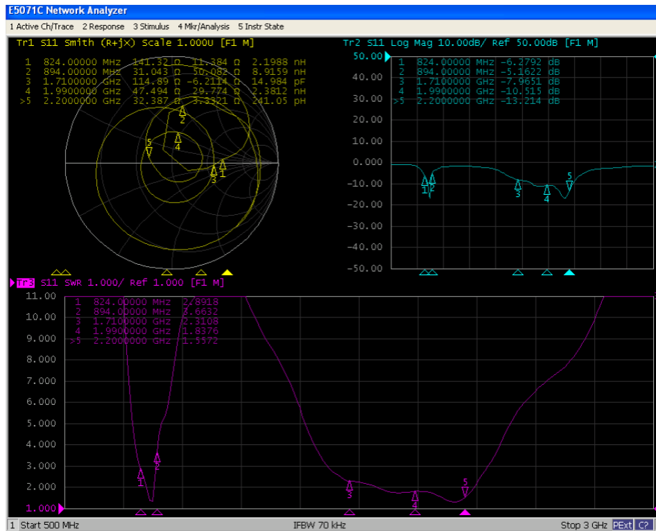
VSWR &amp; Return Loss (GSM2/3/5/8 LTE B2/4/5/66 WCDMA 2/4/5)
