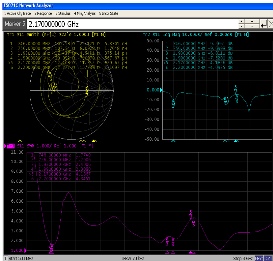
VSWR &amp; Return Loss (LTE B13)
