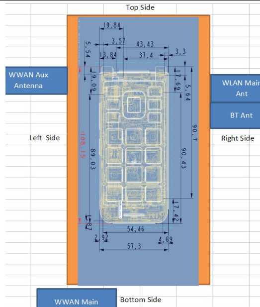
Antenna location
