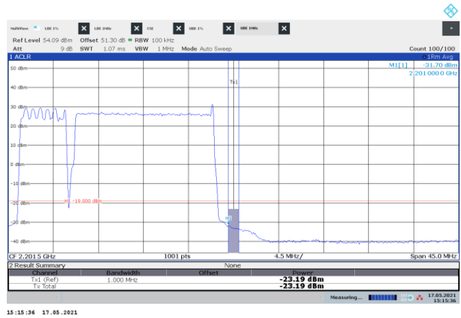
Figure 8.3-160: Conducted emission 1 MHz away from the upper band edge
