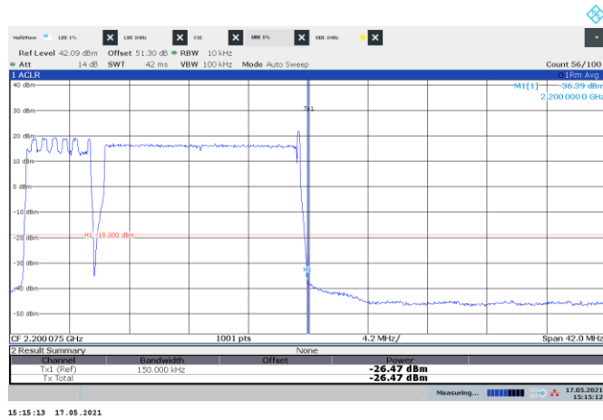
Figure 8.3-159: Conducted emission at the upper band edge
