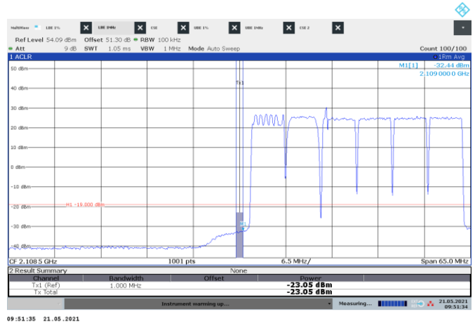
Figure 8.3-166: Conducted emission 1 MHz away from the lower band edge
