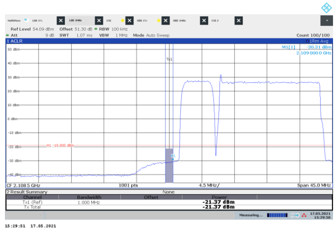
Figure 8.3-186: Conducted emission 1 MHz away from the lower band edge
