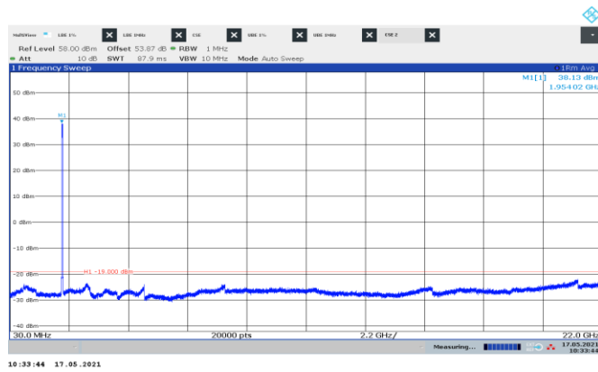
Figure 8.5-46: Conducted spurious emissions of 3xNR 10 MHz contiguous mid channels, multi-carrier operation
