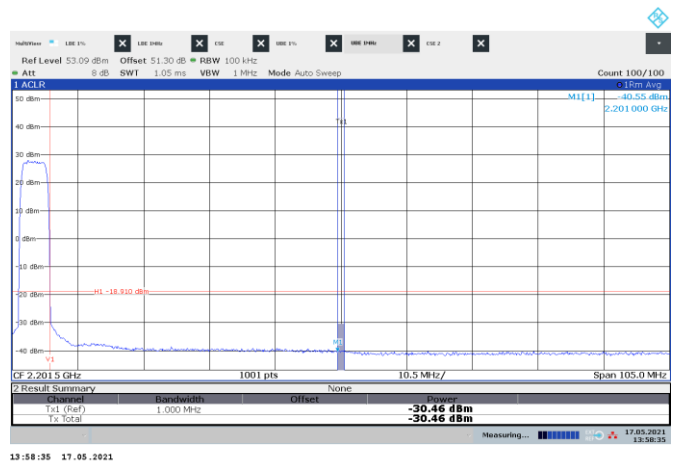
Figure 8.3-148: Conducted emission 1 MHz away from the upper band edge
