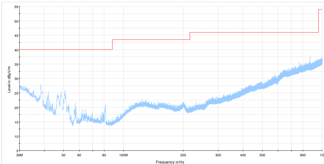
RE 30 MHz to 1 GHz Preview Result 1-PK+ FCC Part 15 Limit - Class B, QP, 3 m
