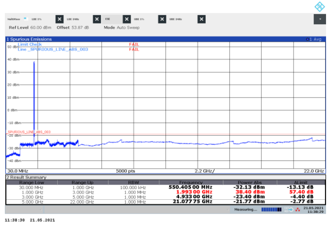
Figure 8.5-39: Conducted spurious emissions of 2xNR 10 MHz non-contiguous channels, multi-carrier operation
