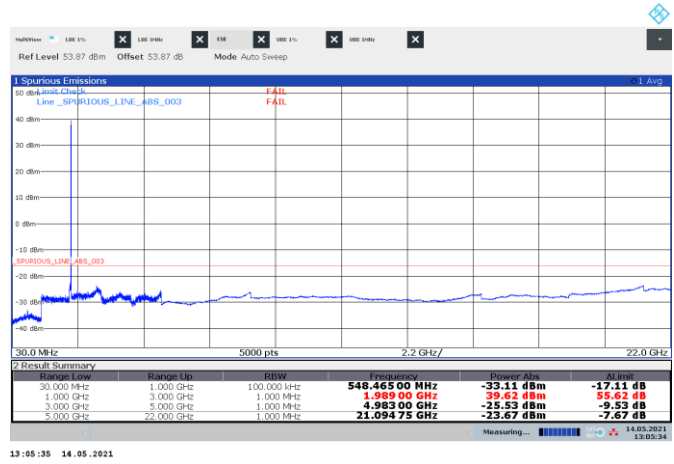
Figure 8.5-31: Conducted spurious emissions of NR 10 MHz top channel, single carrier operation
