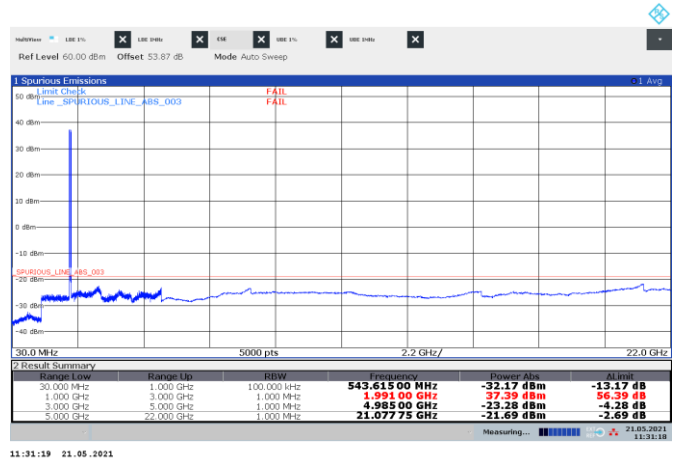
Figure 8.5-14: Conducted spurious emissions of 2xLTE 10 MHz (non-contiguous), multi-carrier operation
