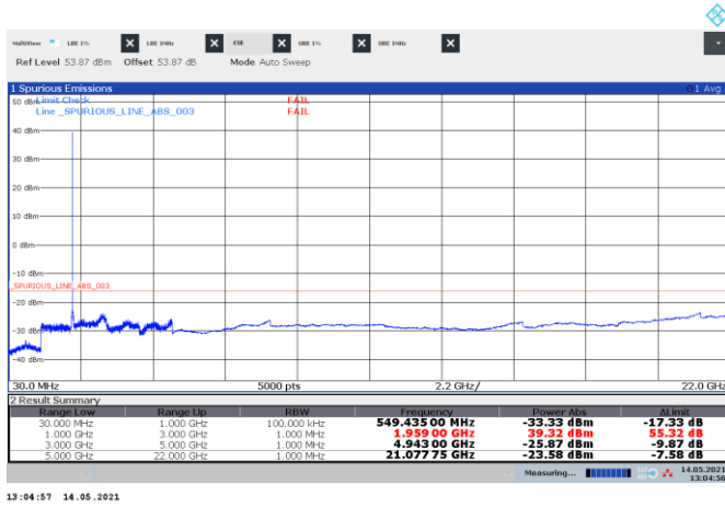
Figure 8.5-30: Conducted spurious emissions of NR 10 MHz mid channel, single carrier operation
