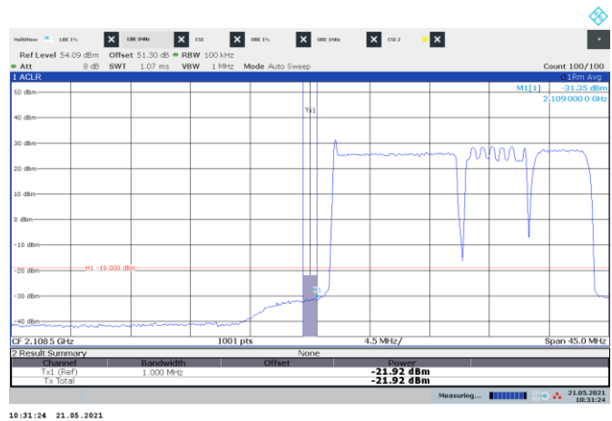
Figure 8.3-154: Conducted emission 1 MHz away from the lower band edge
