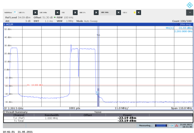
Figure 8.3-172: Conducted emission 1 MHz away from the upper band edge
