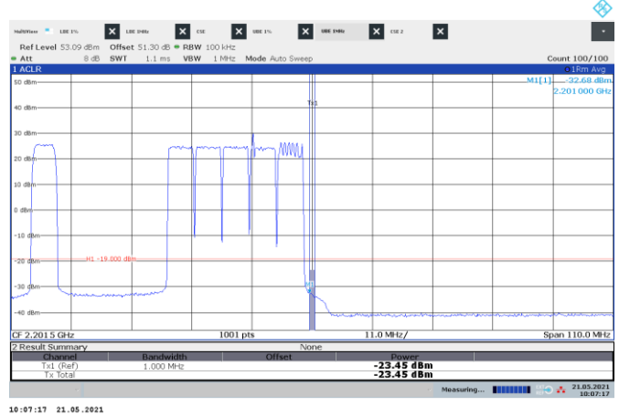
Figure 8.3-168: Conducted emission 1 MHz away from the upper band edge
