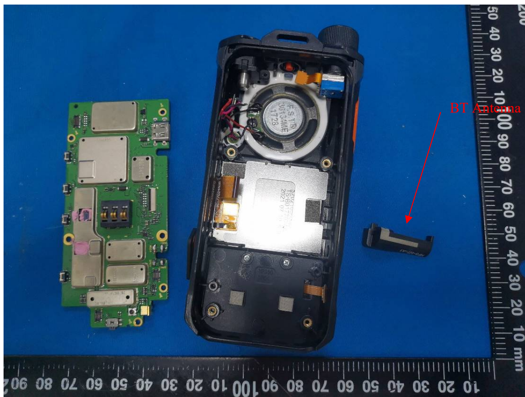
BT Antenna
