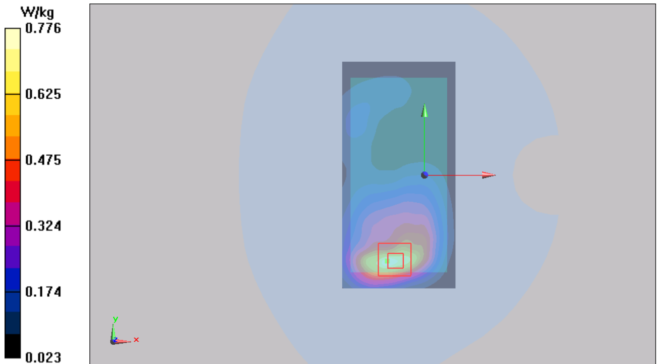
Figure 177 Body, Back Side, LTE Band 2 1RB Channel 18900
