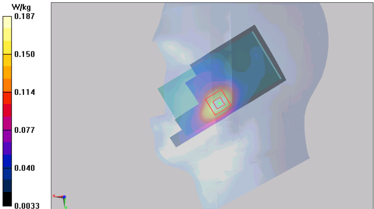
Figure 192 Right Hand Touch Cheek LTE Band 2 50%RB Channel 19100
