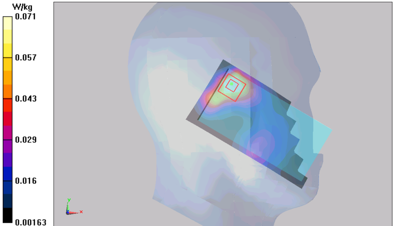
Figure 189 Left Hand Tilt 15° LTE Band 2 50%RB Channel 19100
