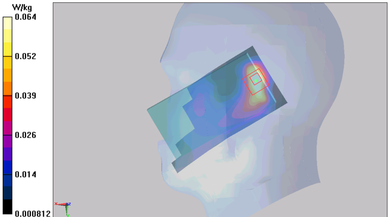
Figure 195 Right Hand Tilt 15° LTE Band 2 50%RB Channel 19100
