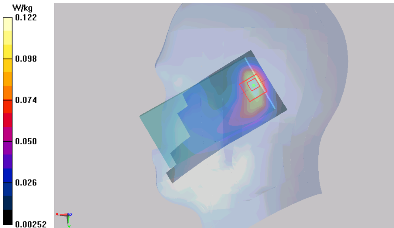
Figure 175 Right Hand Tilt 15° LTE Band 2 1RB Channel 18700
