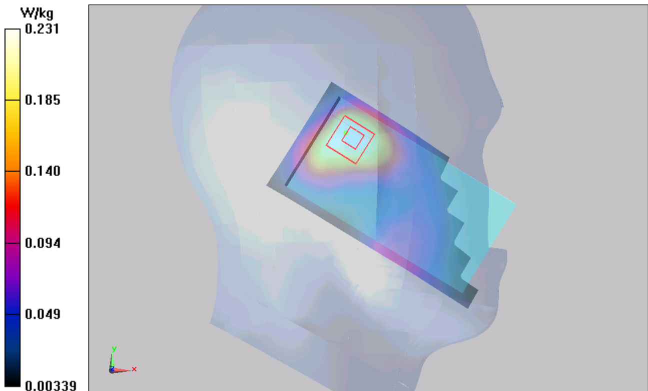
Figure 236 Left Hand Tilt 15^\circ LTE Band 4 50%RB Channel 20300
