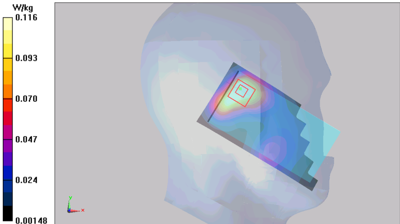
Figure 169 Left Hand Tilt 15° LTE Band 2 1RB Channel 18700
