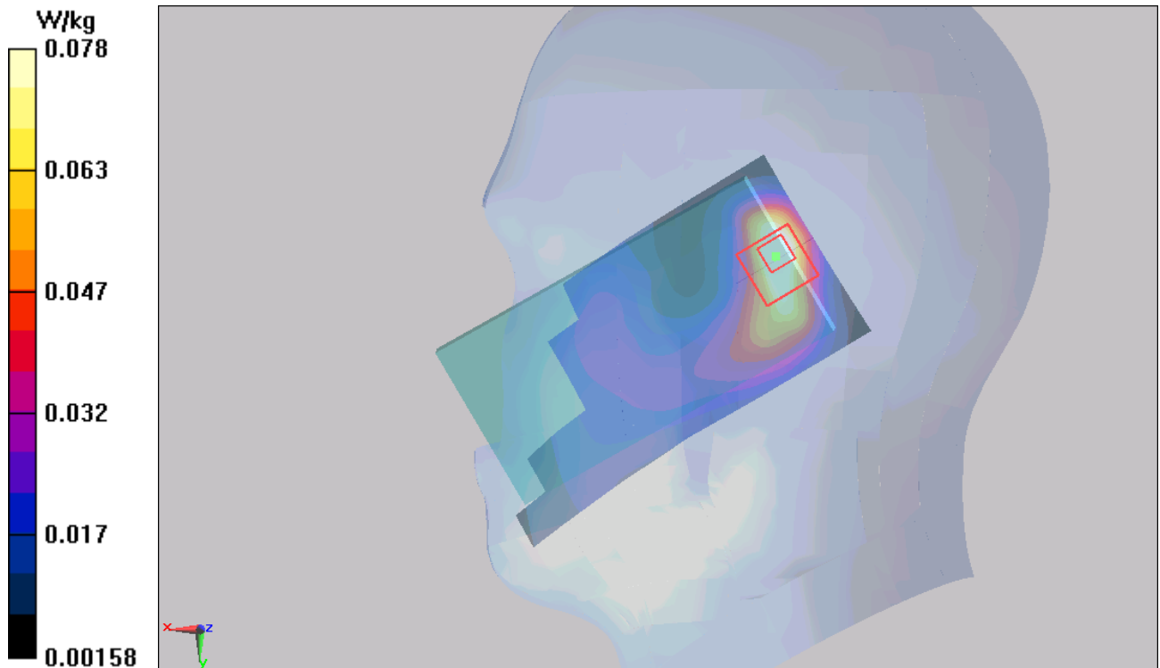
Figure 173 Right Hand Tilt 15° LTE Band 2 1RB Channel 19100
