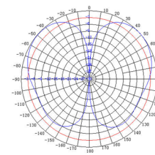
2.4 GHz Vertical Plane
