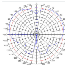
5 GHz Vertical Plane
