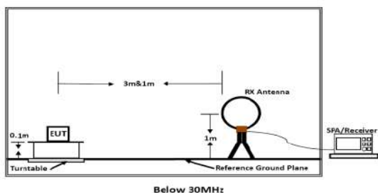
Figure 1. Below 30MHz
