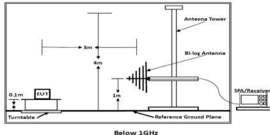
Figure 2. 30MHz to 1GHz
