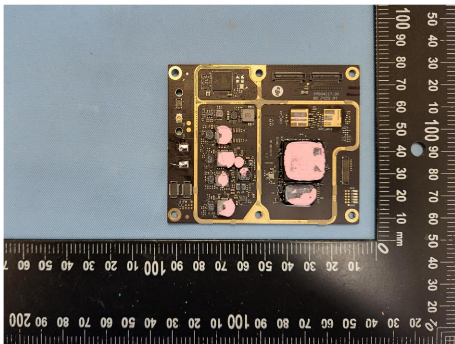
Internal View of EUT-36
