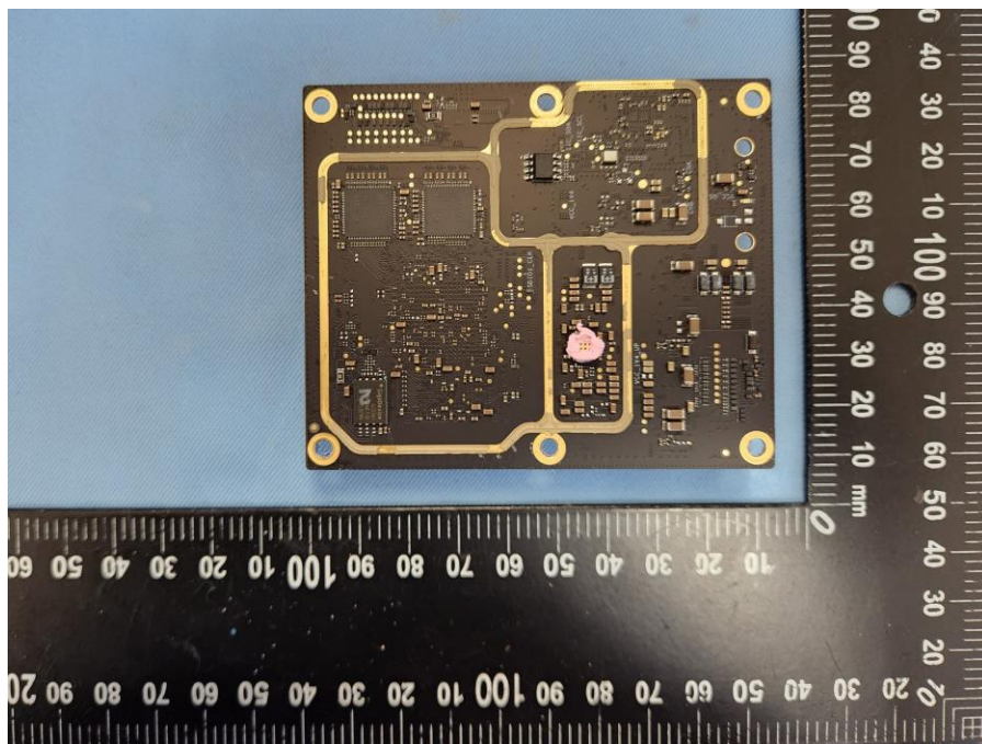
Internal View of EUT-38
