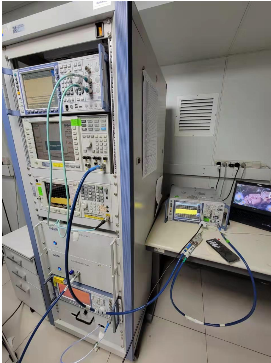
RF Conducted Test setup (GSM/WCDMA/LTE)
