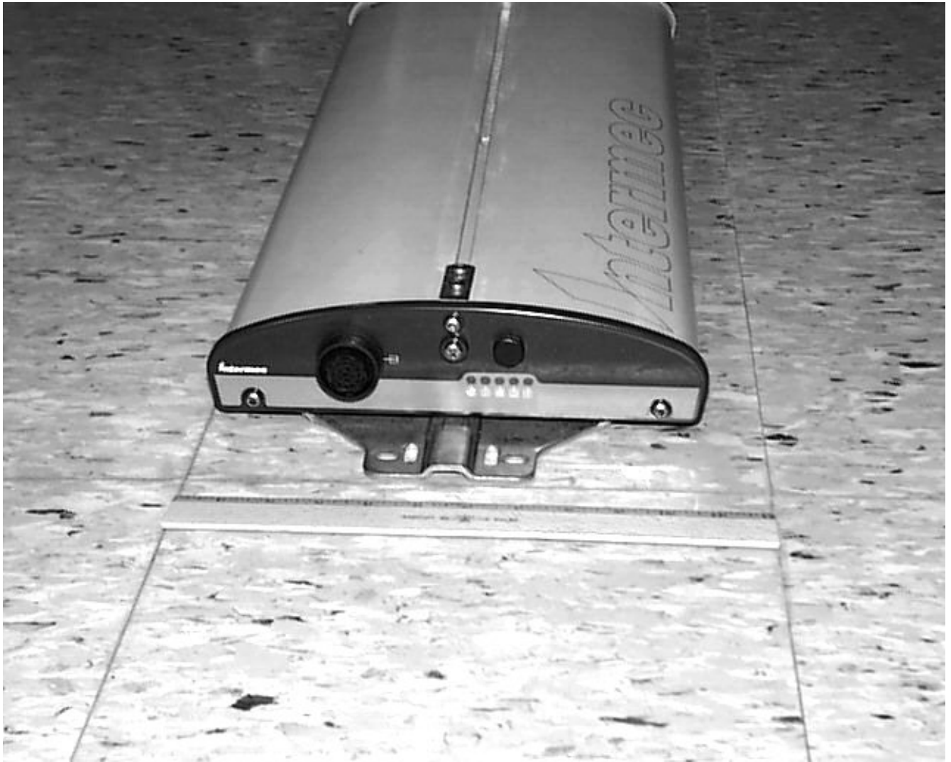
End cap view of IV6 (collocated radio inside) Single connector provides power and I/O functions
