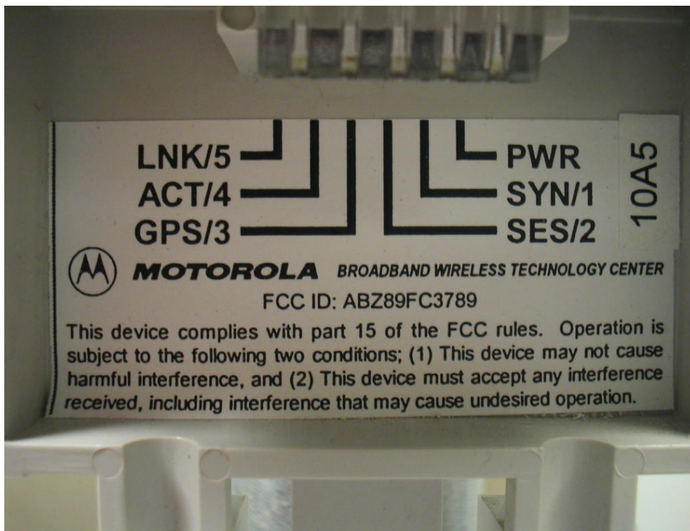
900MHz Canopy Radio Mounted in Chassis – Radio Label with FCC Identifier
