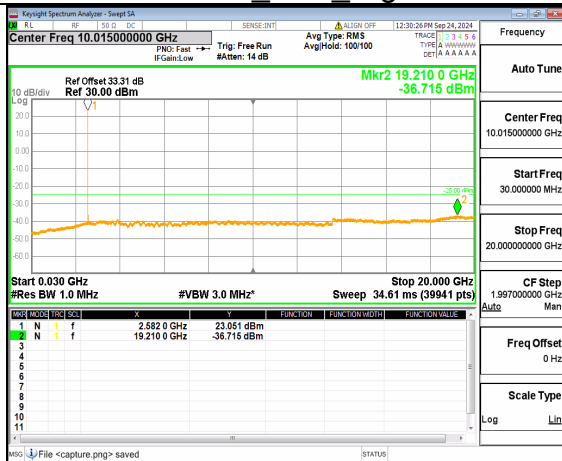
n38 (30MHz-20GHz) 30M DFT-s-OFDM BPSK Inner 1RB Left Mid
