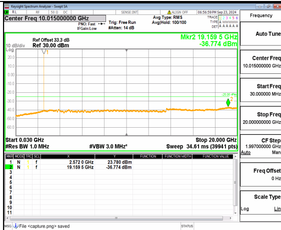
n38 (30MHz-20GHz) 30M DFT-s-OFDM QPSK Inner 1RB Left Low
