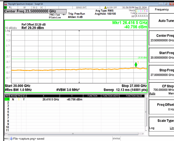
n38 (20GHz-27GHz) 15M DFT-s-OFDM QPSK Inner_1RB Left Low
