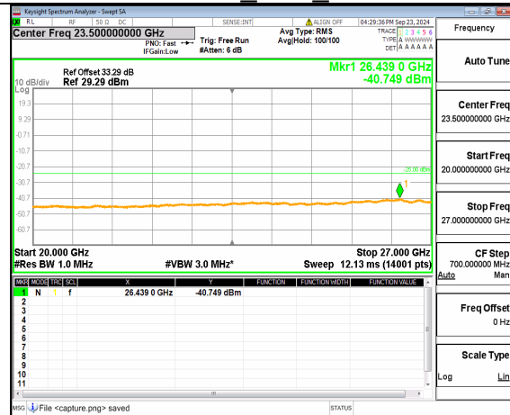
n38 (20GHz-27GHz) 20M DFT-s-OFDM QPSK Inner 1RB Right Low
