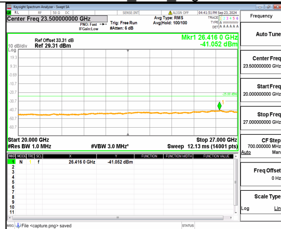
n38 (20GHz-27GHz) 20M DFT-s-OFDM BPSK Inner 1RB Left Mid
