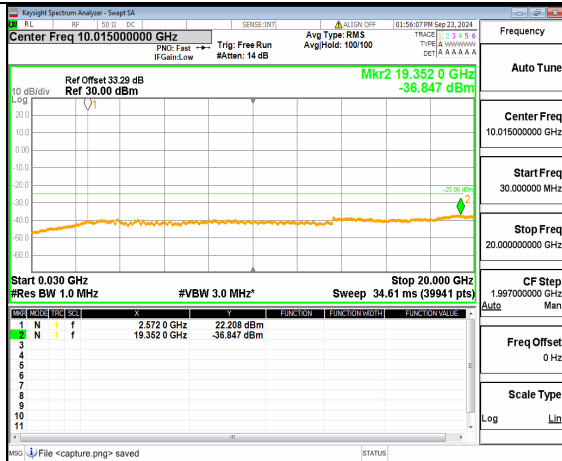
n38 (30MHz-20GHz) 15M DFT-s-OFDM QPSK Inner_1RB Left Low
