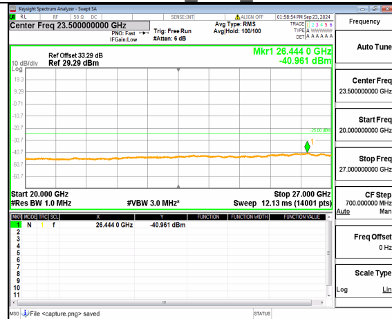
n38 (20GHz-27GHz) 15M DFT-s-OFDM QPSK Inner_1RB Right Low
