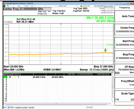
n38 (20GHz-27GHz) 15M DFT-s-OFDM BPSK Inner_1RB Left Mid
