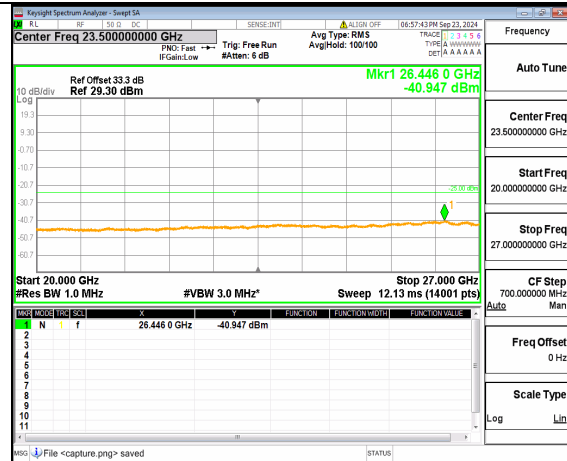
n38 (20GHz-27GHz) 30M DFT-s-OFDM QPSK Inner 1RB Left Low
