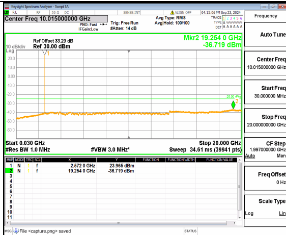
n38 (30MHz-20GHz) 20M DFT-s-OFDM QPSK Inner 1RB Left Low
