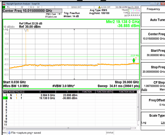
n38 (30MHz-20GHz) 15M DFT-s-OFDM QPSK Inner_1RB Right Low
