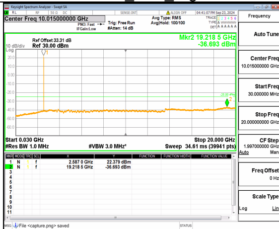
n38 (30MHz-20GHz) 20M DFT-s-OFDM BPSK Inner 1RB Left Mid
