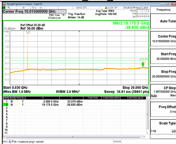
n38 (30MHz-20GHz) 20M DFT-s-OFDM QPSK Inner 1RB Right Low
