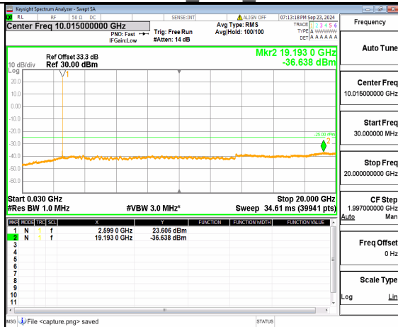
n38 (30MHz-20GHz) 30M DFT-s-OFDM QPSK Inner 1RB Right Low
