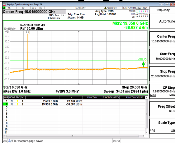
n38 (30MHz-20GHz) 15M DFT-s-OFDM BPSK Inner_1RB Left Mid
