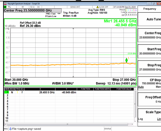
n38 (20GHz-27GHz) 30M DFT-s-OFDM QPSK Inner 1RB Right Low
