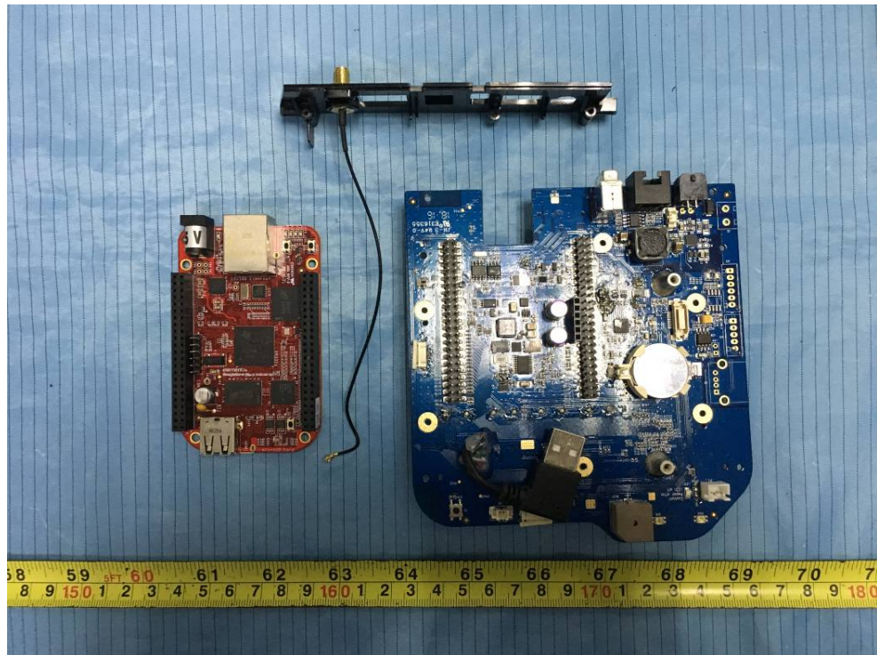
EUT – Cover off View 3
