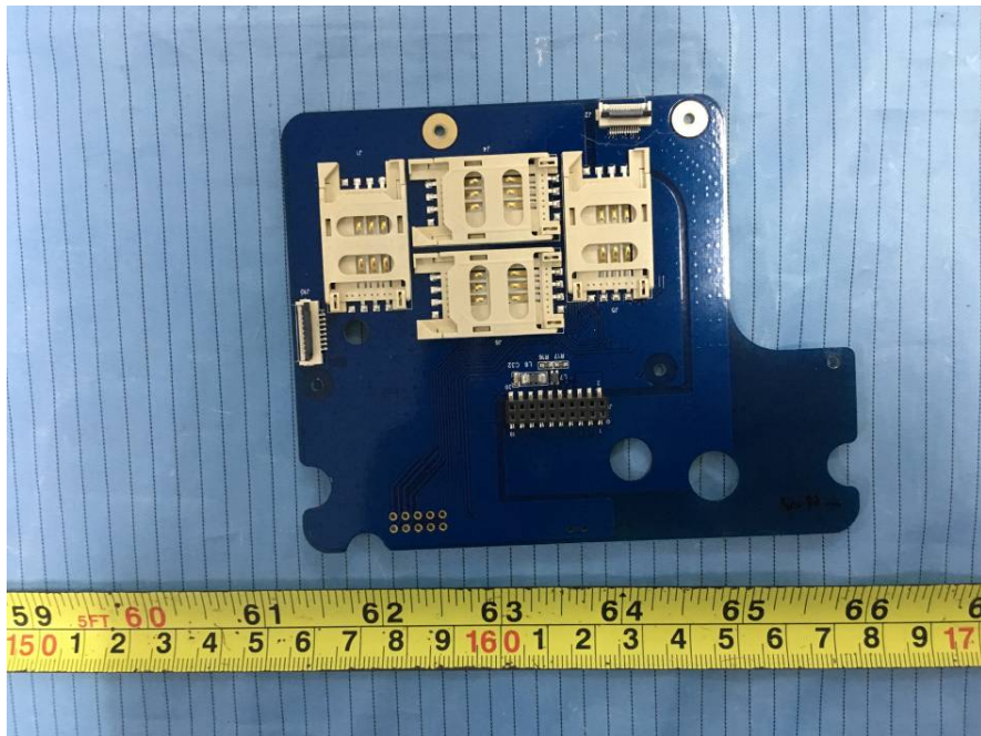
EUT – PCD Main Board Top View
