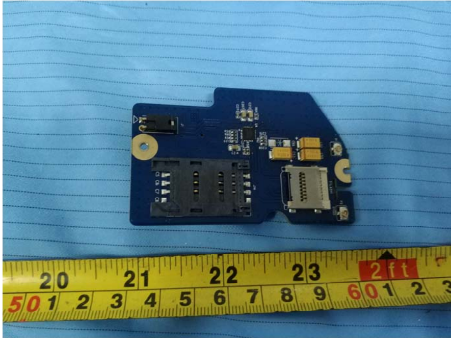
EUT -2G/3G/4G Module Main Board Bottom View
