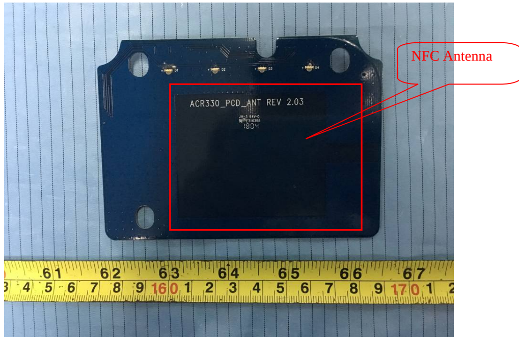
EUT –NFC Antenna Top View
