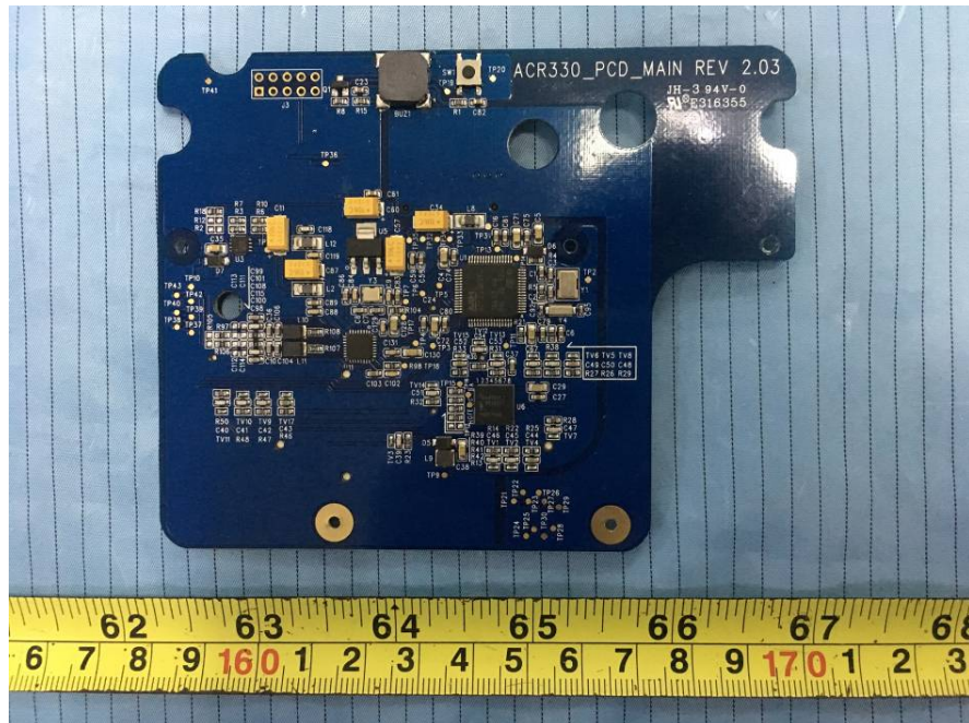
EUT – PCD Main Board Bottom View
