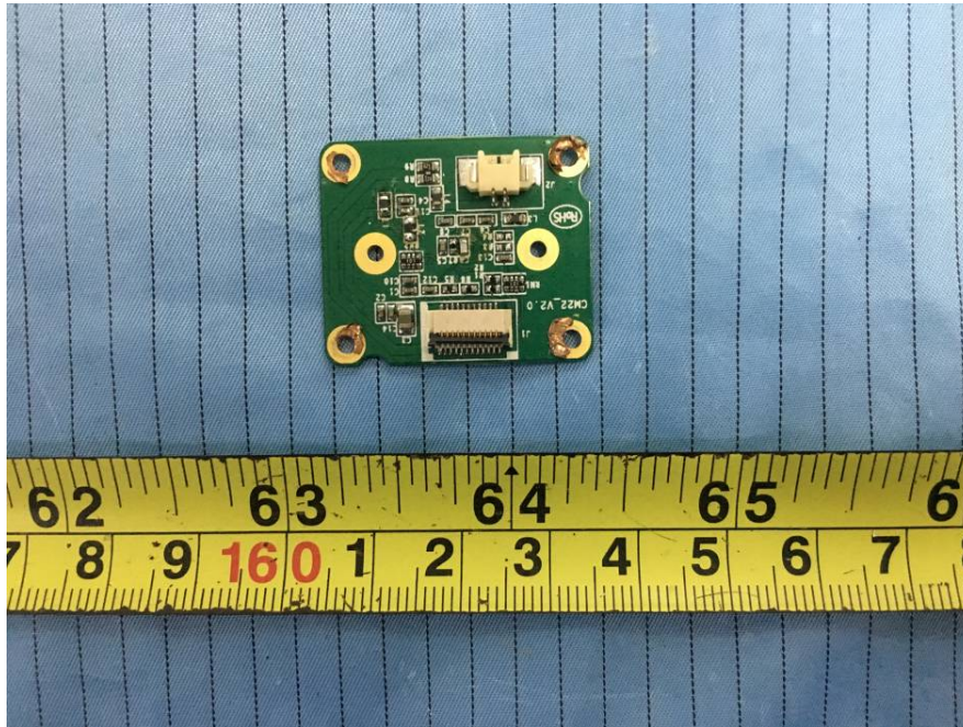
EUT – Sensor Board Bottom View
