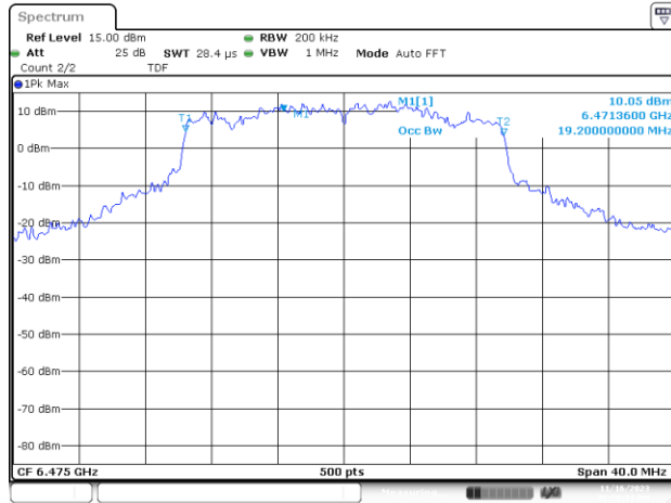
UNII6 SISO B 802.11ax/be20 ch105 6475MHz 99%
