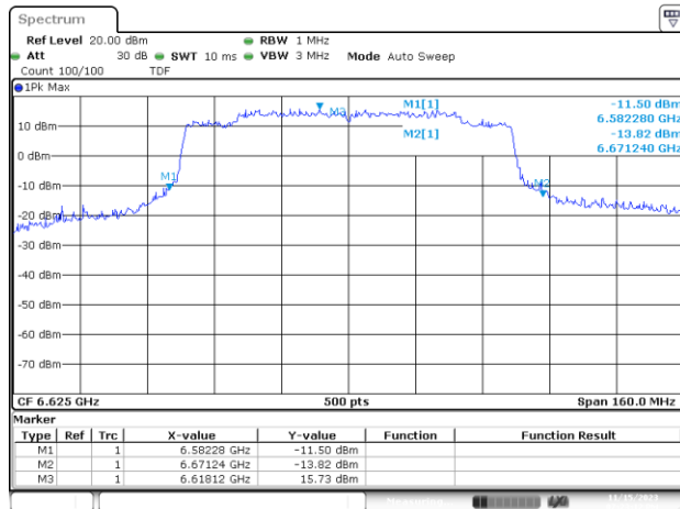
UNII7 SISO A 802.11ax/be80 ch135 6625MHz 99%
