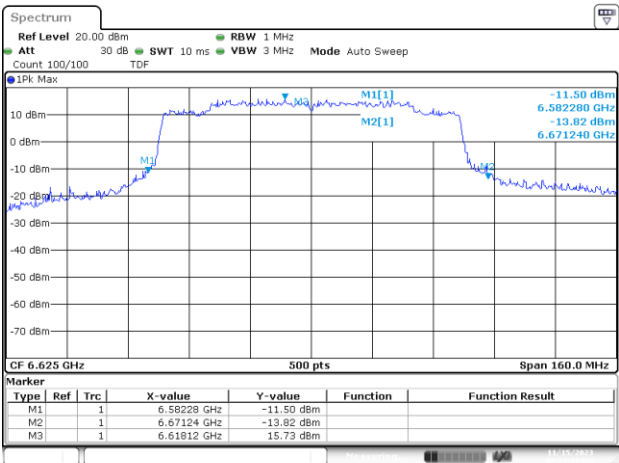
UNII7 SISO A 802.11ax/be80 ch135 6625MHz 26dB
