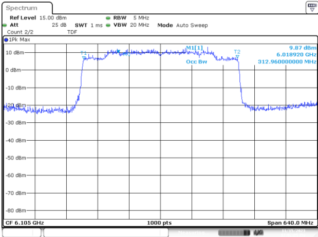
UNII6 SISO A 802.11be320 ch31 6105MHz 99%
