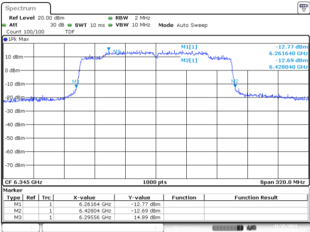
UNII5 SISO A 802.11ax/be160 ch79 6345MHz 26dB
