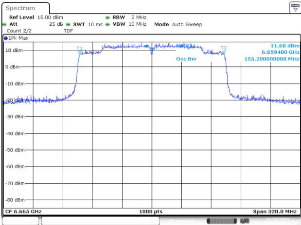
UNII7 SISO A 802.11ax/be160 ch143 6665MHz 99%
