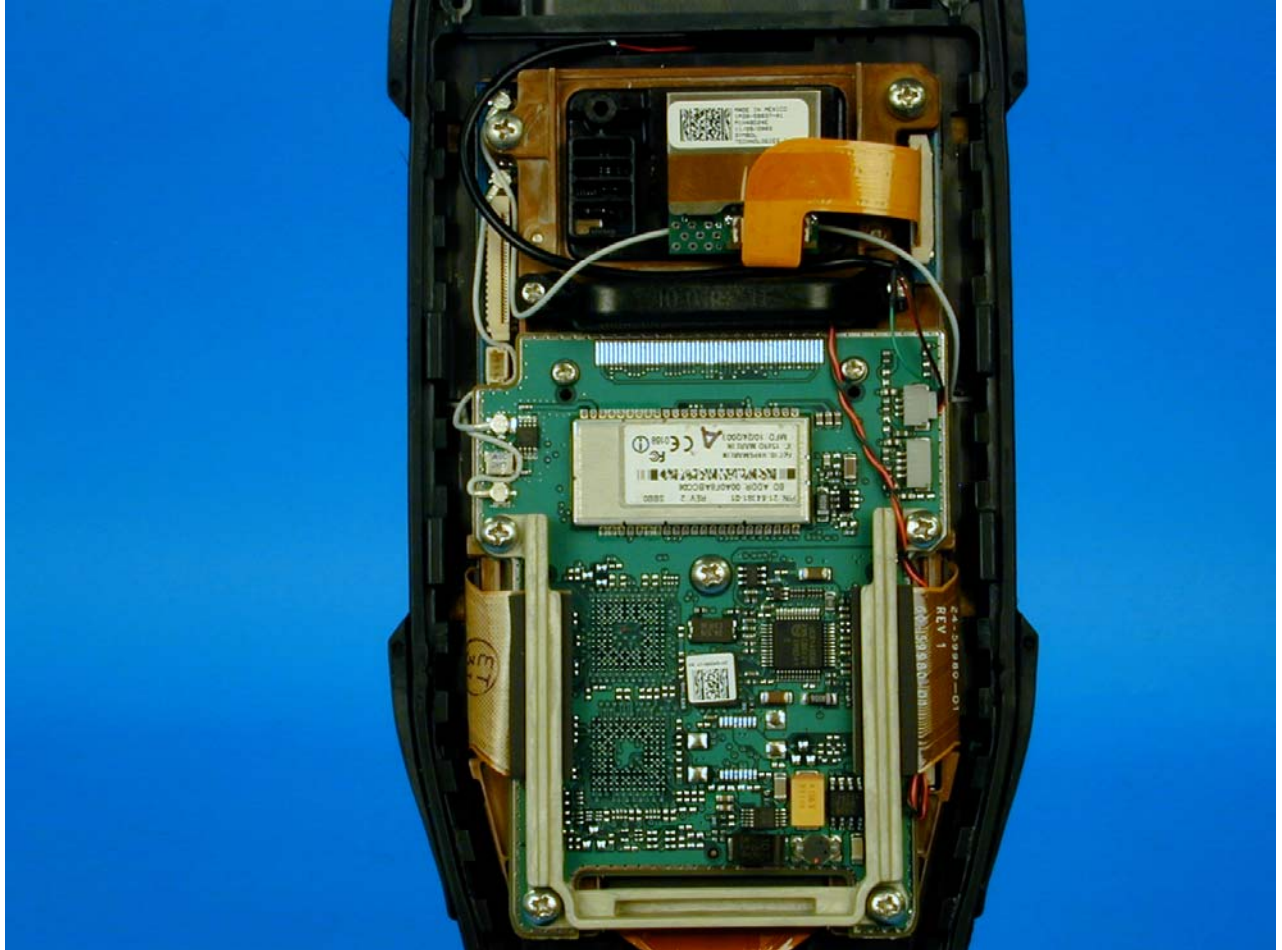
Internal View 4
