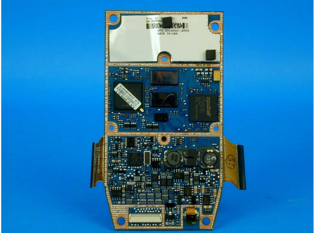
Internal View 7
