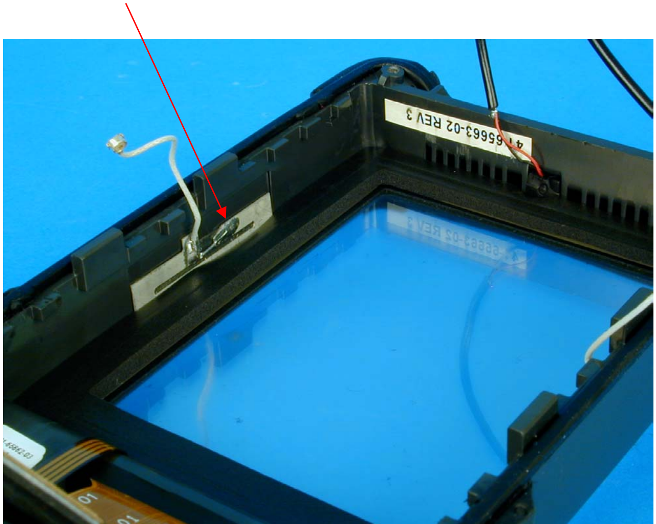
Antenna View 2
