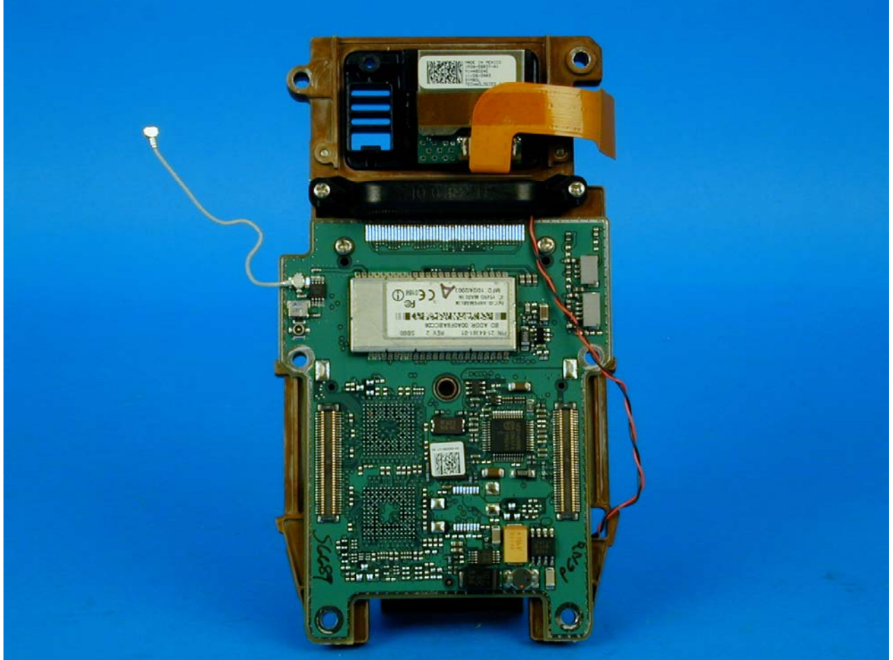
Internal View 5
