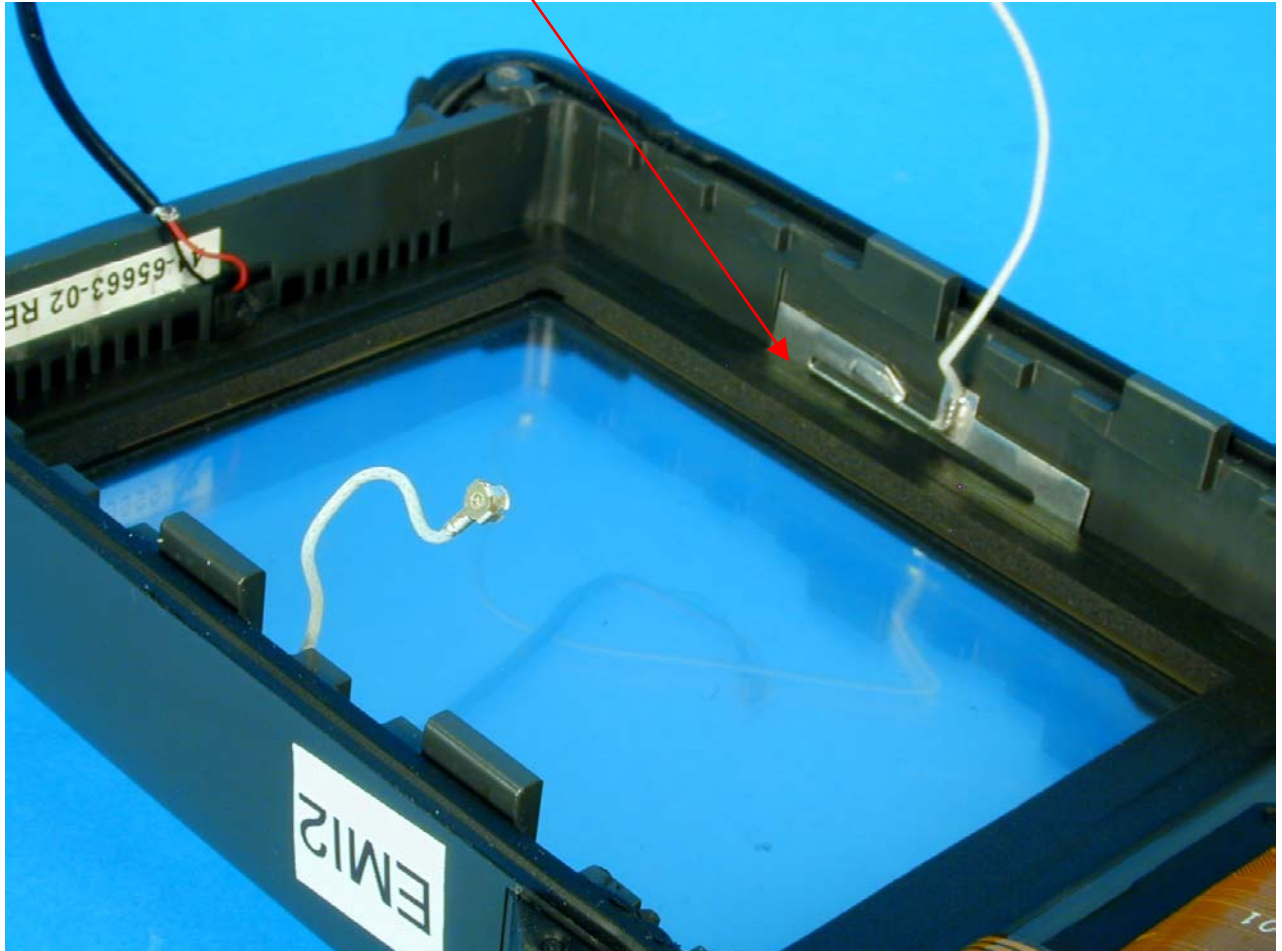
Antenna View 1
