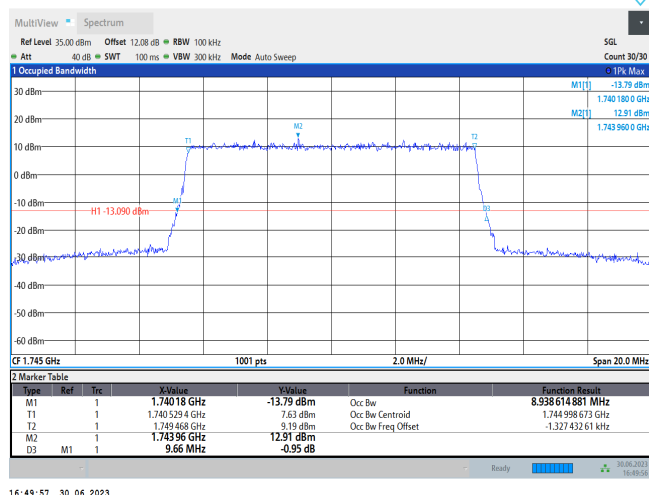
Band66-10MHz-64QAM-132322-50RB#0
