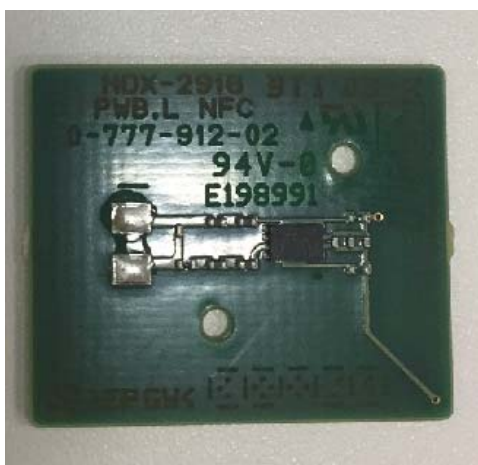
NFC mount
