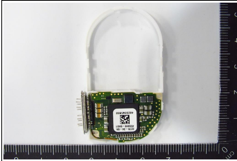
PC-Board 2270 Top View
