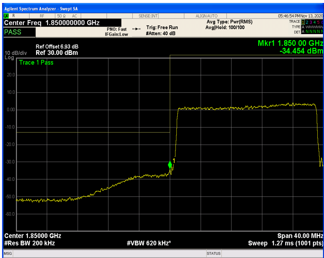
LTE Band2 QAM16 BW=20MHz Channel=18700 RB Size=1 Position=#Max
