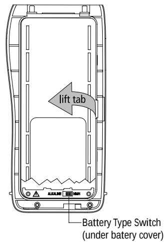
Figure 2-2: Removing the Battery Tray Cover
