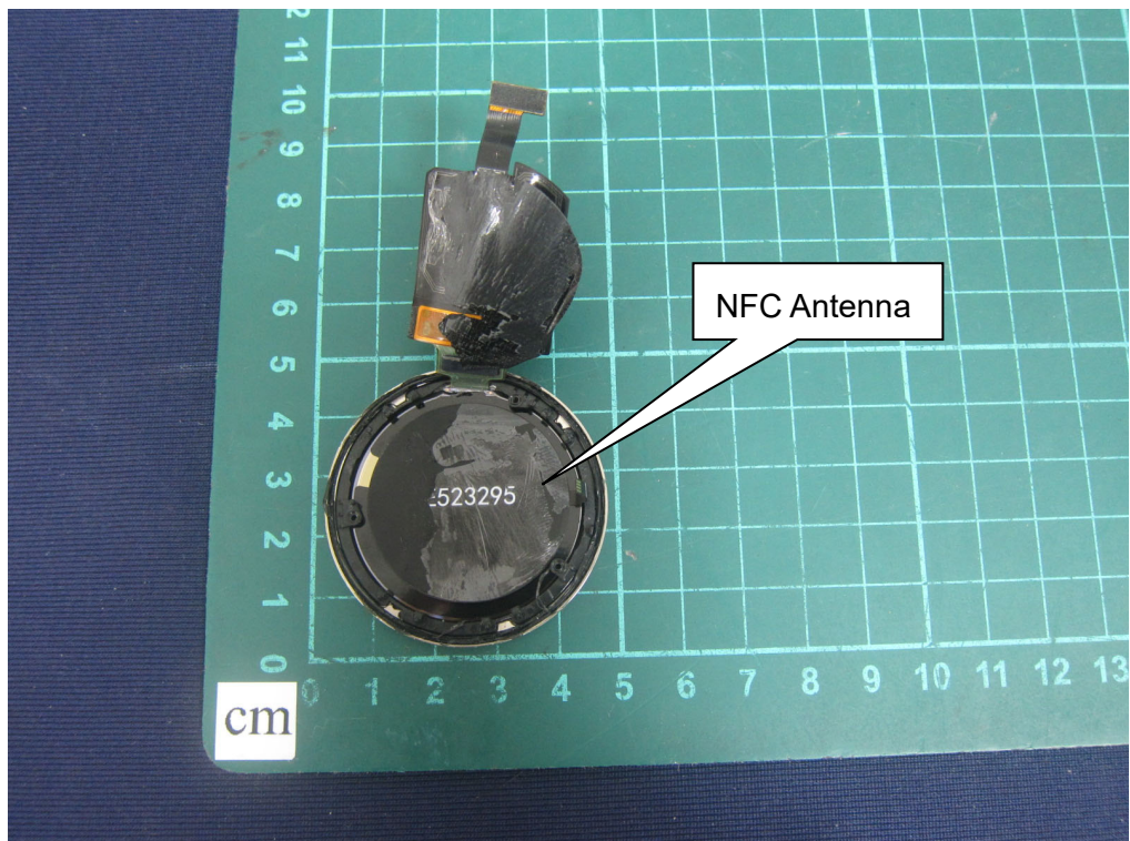
(28) EUT Photo
