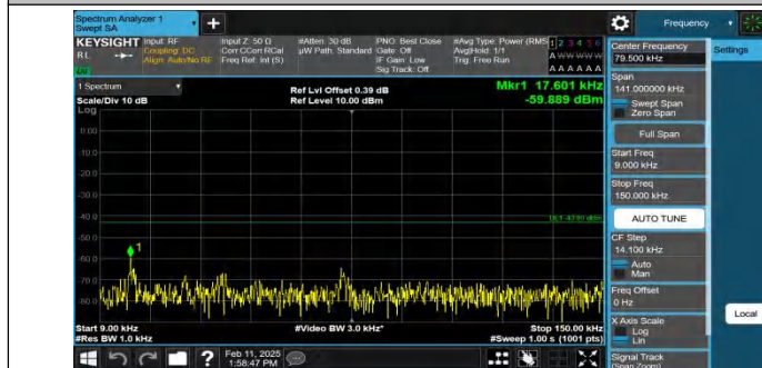
Band2-20MHz-QPSK-18700-1RB#0-0.009~0.15-PASS
