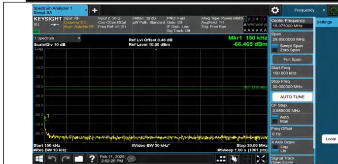
Band2-20MHz-QPSK-19100-1RB#99-0.15~30-PASS
