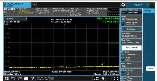
Band2-10MHz-QPSK-19150-1RB#49-30~1000-PASS
