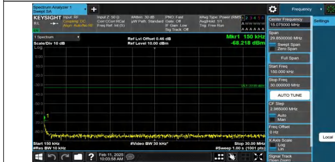
Band2-15MHz-QPSK-19125-1RB#74-0.15~30-PASS
