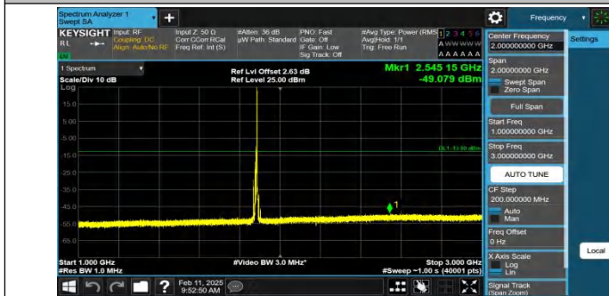
Band2-10MHz-QPSK-18900-1RB#49-1000~3000-PASS
