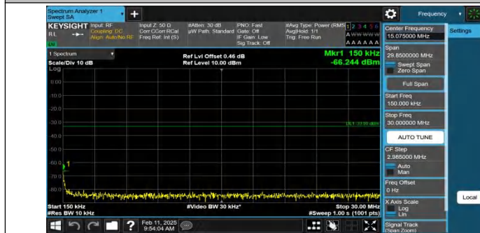
Band2-10MHz-QPSK-19150-1RB#49-0.15~30-PASS
