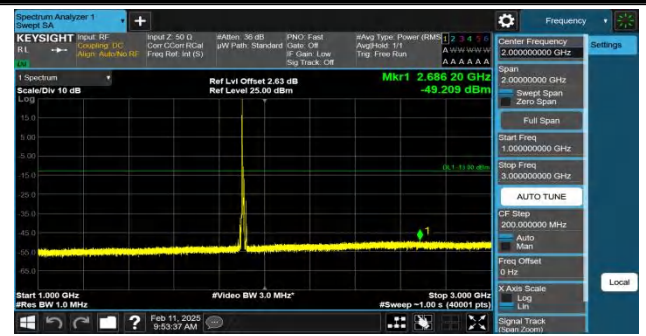
Band2-10MHz-QPSK-19150-1RB#0-1000~3000-PASS
