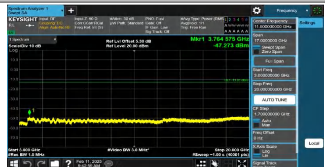
Band2-5MHz-QPSK-18900-1RB#24-3000~20000-PASS
