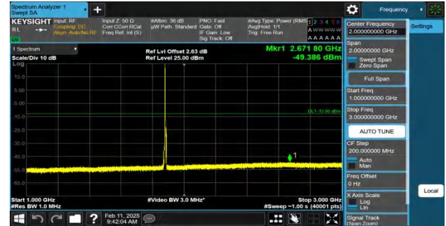
Band2-5MHz-QPSK-18900-1RB#0-1000~3000-PASS
