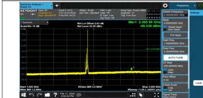
Band2-20MHz-QPSK-19100-1RB#99-1000~3000-PASS
