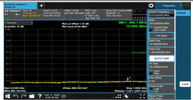
Band2-10MHz-QPSK-18900-1RB#49-30~1000-PASS
