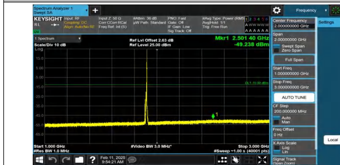
Band2-10MHz-QPSK-19150-1RB#49-1000~3000-PASS
