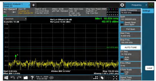
Band2-10MHz-QPSK-18900-1RB#49-0.009~0.15-PASS
