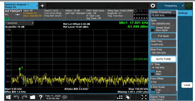
Band2-10MHz-QPSK-19150-1RB#49-0.009~0.15-PASS
