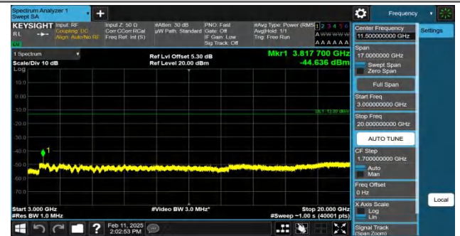
Band2-20MHz-QPSK-19100-1RB#99-3000~20000-PASS
