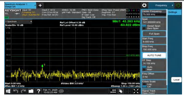
Band2-15MHz-QPSK-18900-1RB#74-0.009~0.15-PASS
