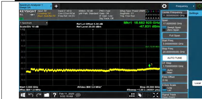
Band2-10MHz-QPSK-18900-1RB#0-3000~20000-PASS
