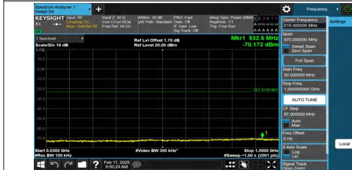
Band2-10MHz-QPSK-18650-1RB#0-30~1000-PASS
