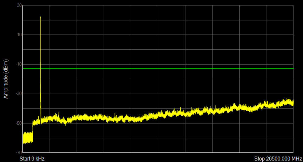
Band66 QPSK BW=10MHz Channel=132622 RB Size=50 Position=#0
