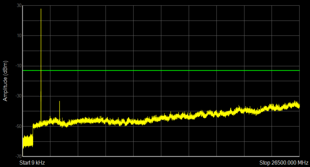
Band66 QPSK BW=5MHz Channel=132647 RB Size=1 Position=#0
