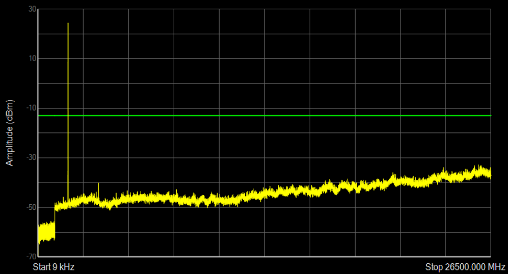
Band66 QAM16 BW=3MHz Channel=132657 RB Size=15 Position=#0
