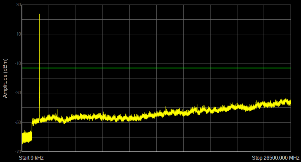
Band66 QAM16 BW=5MHz Channel=132322 RB Size=25 Position=#0
