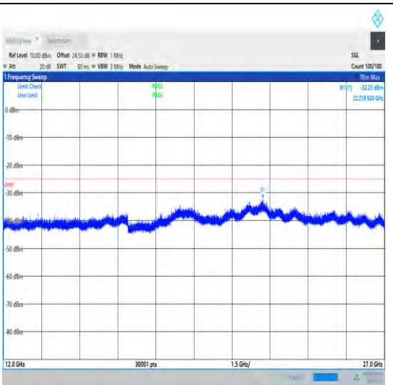
1-N41-30-100-L-1-DFT-PI2BPSK-Inner_1RB _Left-1@1-12000-27000-Ant1-22219.50--32. 23--25-PASS
