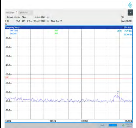
1-N41-30-100-M-1-DFT-PI2BPSK-Inner_1RB _Left-1@1-0.009-0.15-Ant1-0.13--72.77--55- PASS
