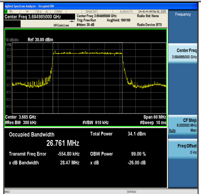
NTNV-n48-PC3-30-30-H-DFT-BPSK-Outer_Full-Ant1- PASS
