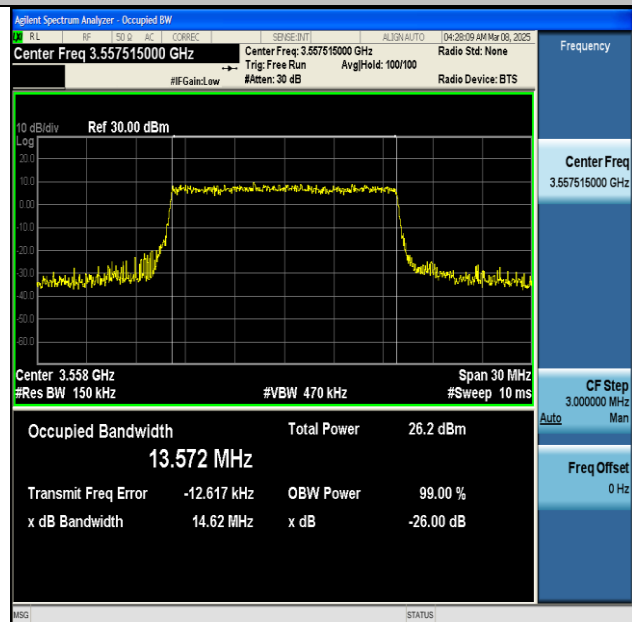
NTNV-n48-PC3-30-15-L-CP-256QAM-Outer_Full-Ant1-PASS
