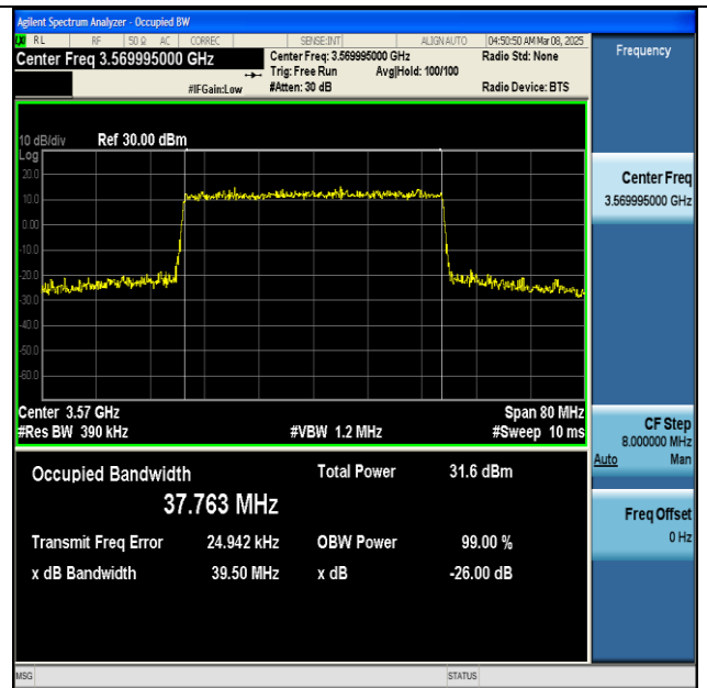
NTNV-n48-PC3-30-40-L-CP-QPSK-Outer_Full-Ant1-PASS
