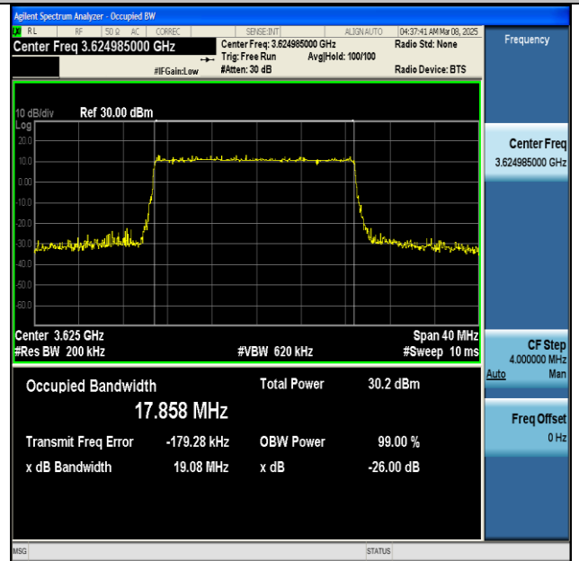
NTNV-n48-PC3-30-20-M-DFT-256QAM-Outer_Full-Ant1- PASS
