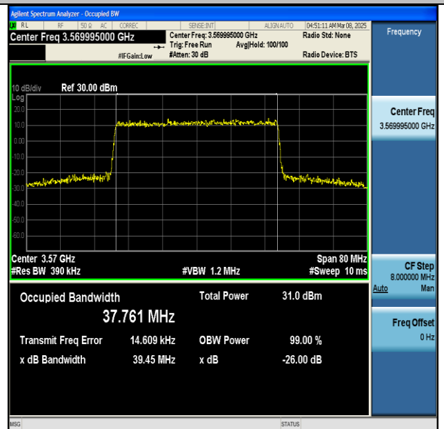
NTNV-n48-PC3-30-40-L-CP-64QAM-Outer_Full-Ant1-PASS
