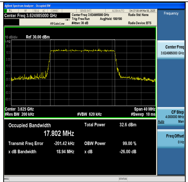
NTNV-n48-PC3-30-20-M-DFT-16QAM-Outer_Full-Ant1- PASS
