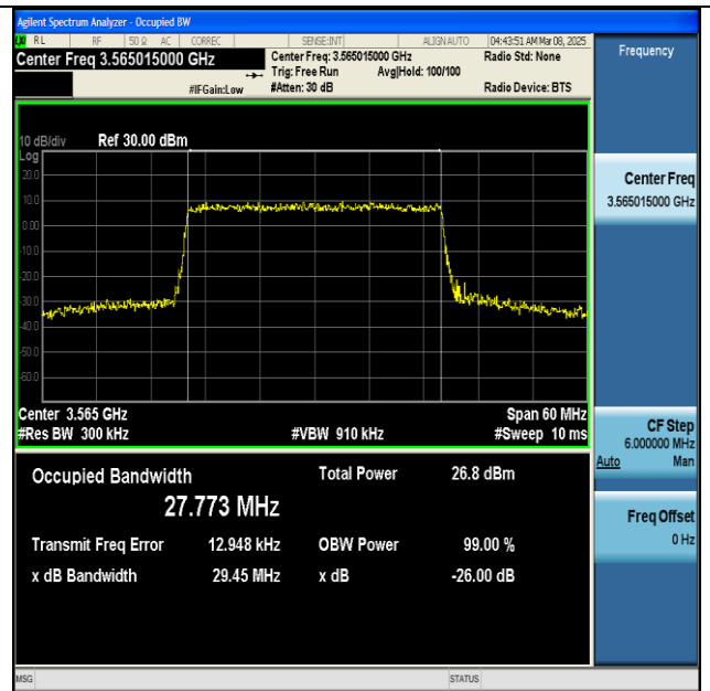
NTNV-n48-PC3-30-30-L-CP-256QAM-Outer_Full-Ant1- PASS
