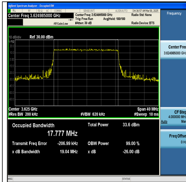
NTNV-n48-PC3-30-20-M-DFT-QPSK-Outer_Full-Ant1- PASS
