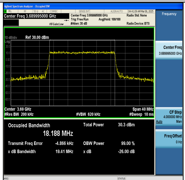
NTNV-n48-PC3-30-20-H-CP-64QAM-Outer_Full-Ant1-PASS
