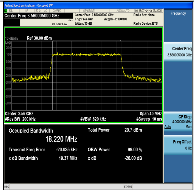
NTNV-n48-PC3-30-20-L-CP-QPSK-Outer_Full-Ant1-PASS
