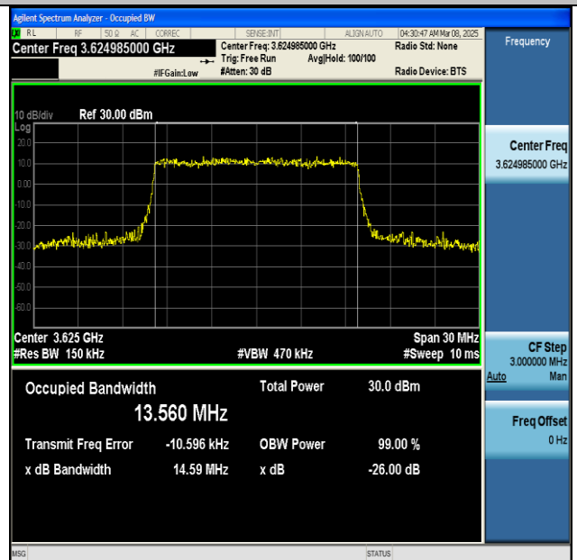
NTNV-n48-PC3-30-15-M-CP-64QAM-Outer_Full-Ant1-PASS
