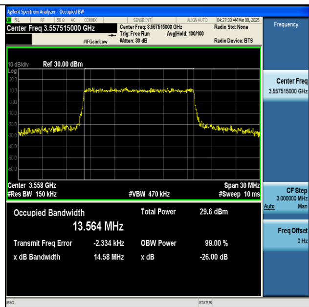
NTNV-n48-PC3-30-15-L-CP-16QAM-Outer_Full-Ant1-PASS
