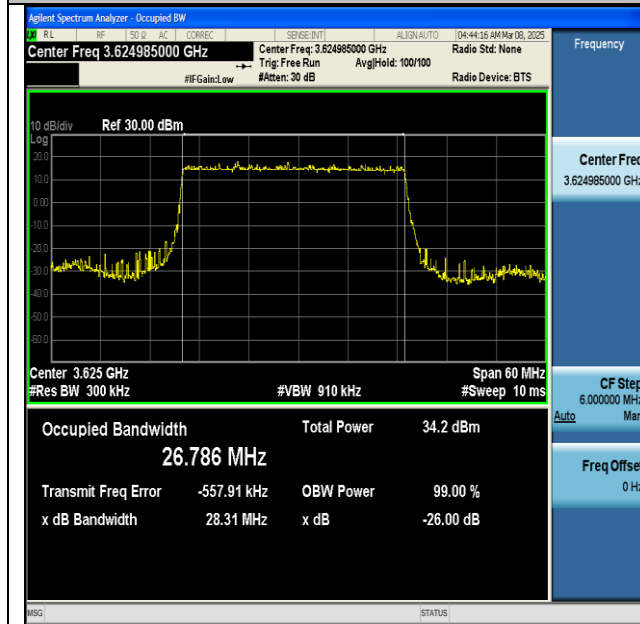
NTNV-n48-PC3-30-30-M-DFT-BPSK-Outer_Full-Ant1- PASS
