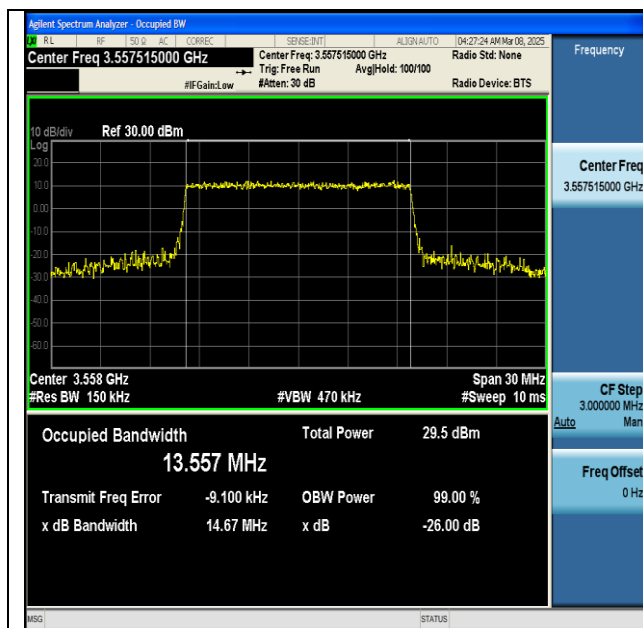
NTNV-n48-PC3-30-15-L-CP-QPSK-Outer_Full-Ant1-PASS
