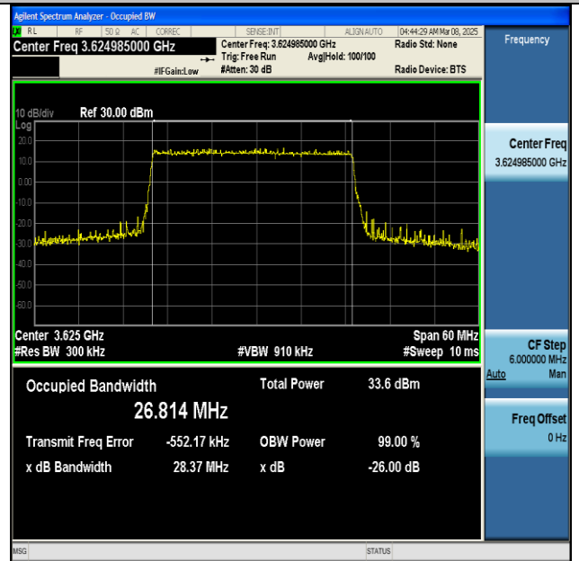
NTNV-n48-PC3-30-30-M-DFT-QPSK-Outer_Full-Ant1- PASS
