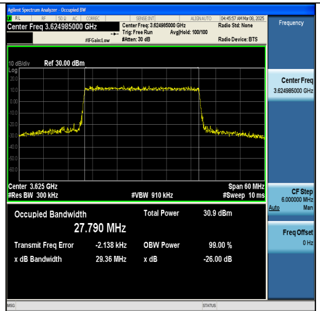
NTNV-n48-PC3-30-30-M-CP-64QAM-Outer_Full-Ant1- PASS
