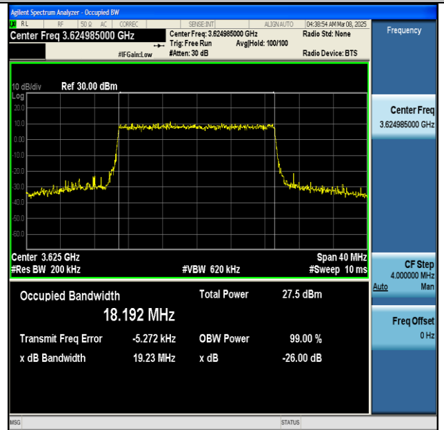
NTNV-n48-PC3-30-20-M-CP-256QAM-Outer_Full-Ant1-PASS
