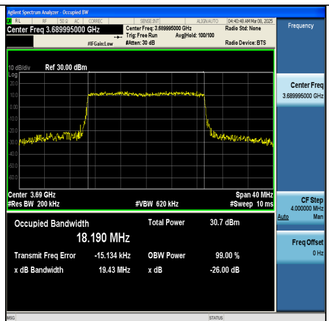
NTNV-n48-PC3-30-20-H-CP-QPSK-Outer_Full-Ant1-PASS
