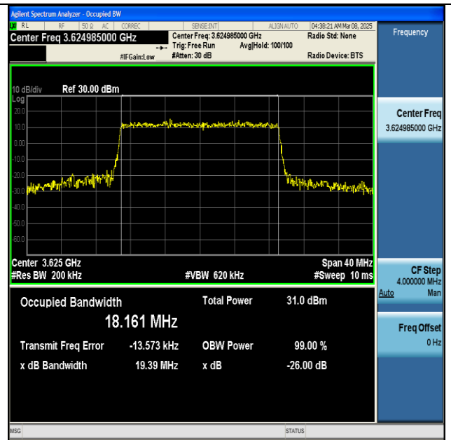
NTNV-n48-PC3-30-20-M-CP-16QAM-Outer_Full-Ant1-PASS
