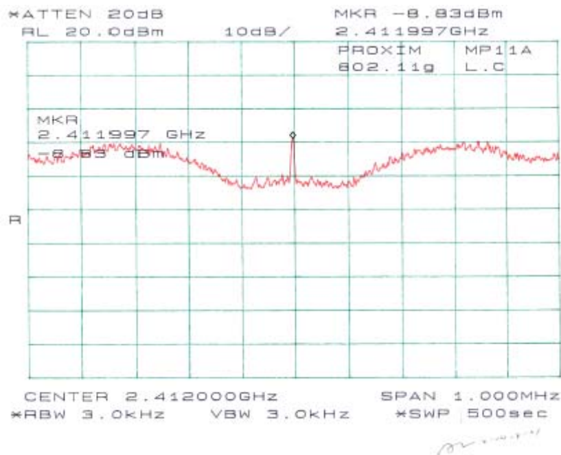
Plots of Power Spectral Density for 802.11g (15.247)
