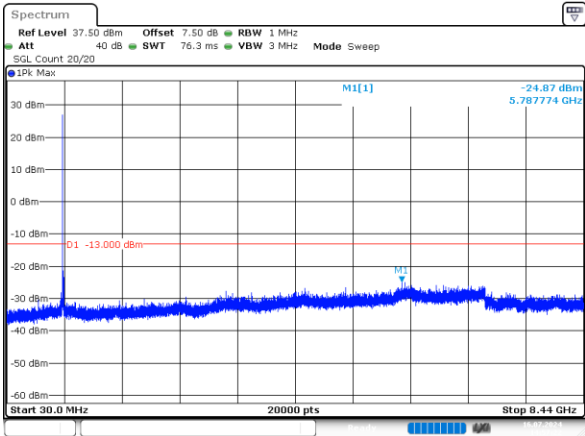
10MHz_High_QPSK_1@0 -24.87dBm
