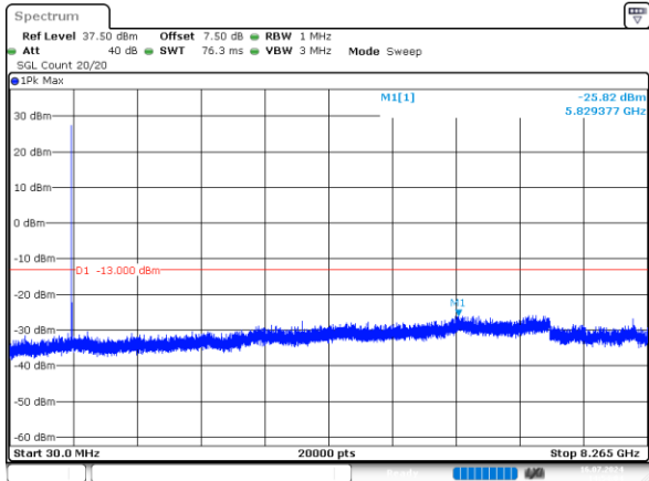
5MHz_Low_QPSK_1@0 -25.82dBm
