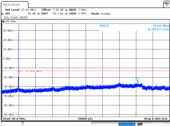
10MHz_Middle_QPSK_1@0 -25.02dBm
