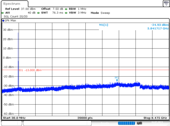
3MHz_High_QPSK_1@0 -24.93dBm
