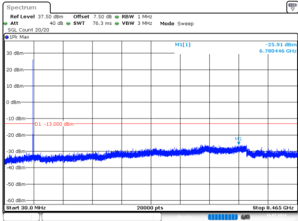
5MHz_High_QPSK_1@0 -25.91dBm
