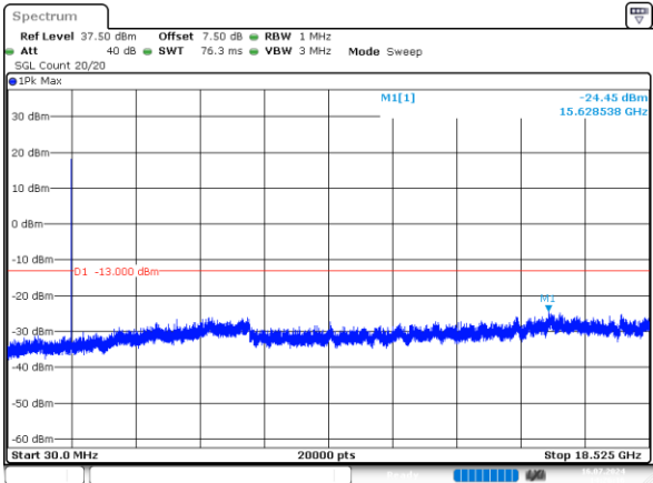
5MHz_Low_QPSK_1@0 -24.45dBm
