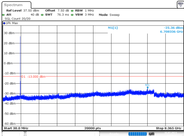
5MHz_Middle_QPSK_1@0 -25.36dBm
