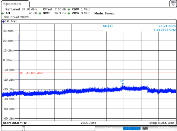
3MHz_Middle_QPSK_1@0 -25.21dBm
