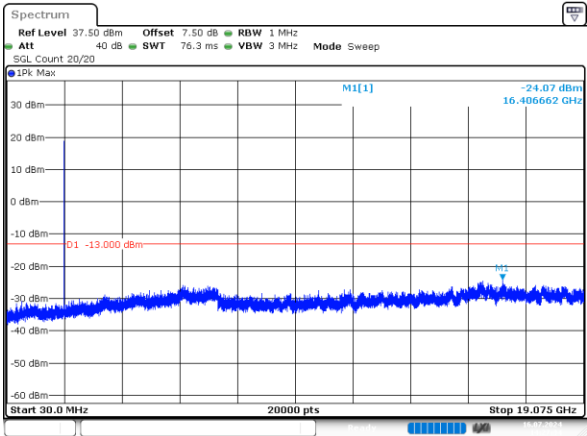
5MHz_High_QPSK_1@0 -24.07dBm
