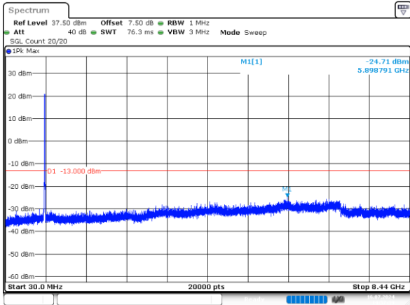
10MHz_High_QPSK_50@0 -24.71dBm
