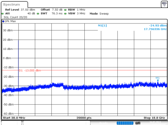
5MHz_Middle_QPSK_1@0 -24.93dBm
