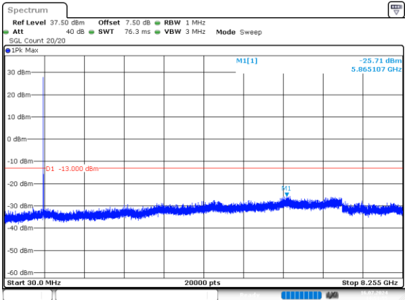
3MHz_Low_QPSK_1@0 -25.71dBm
