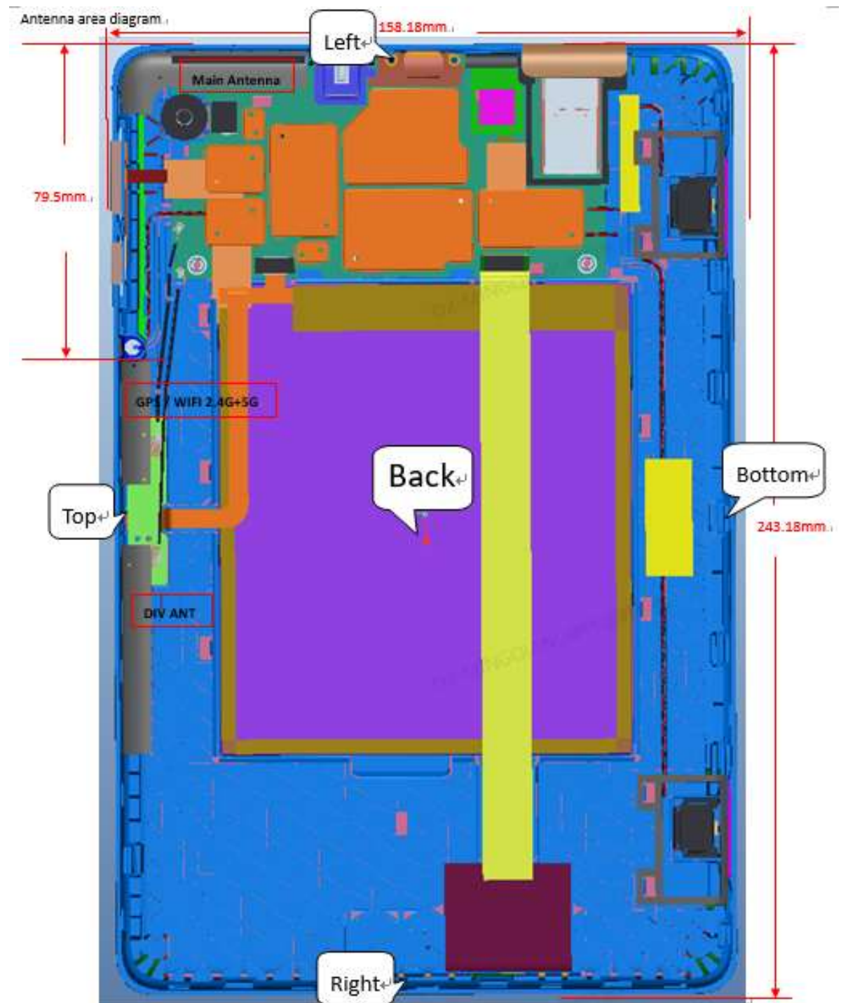
Picture 10: Antenna location
