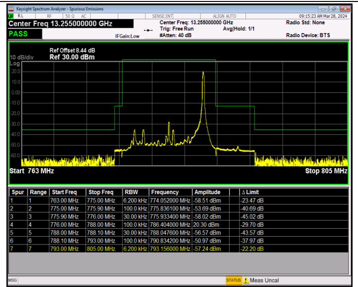
Band13_10MHz_QPSK_23230_1RB#49
