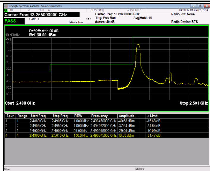
Band41_5MHz_16QAM_39675_1RB#0
