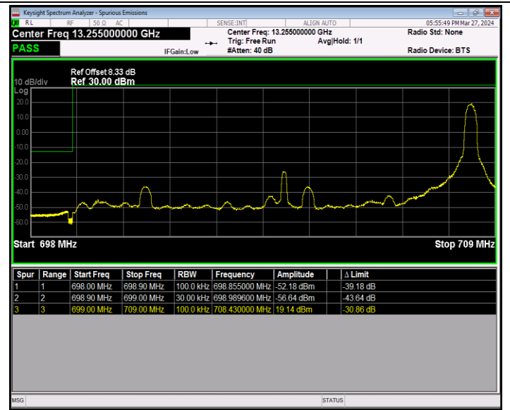
Band12_10MHz_16QAM_23060_1RB#49
