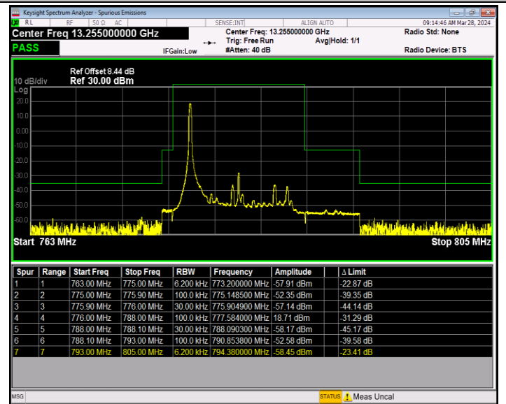
Band13_10MHz_16QAM_23230_1RB#0
