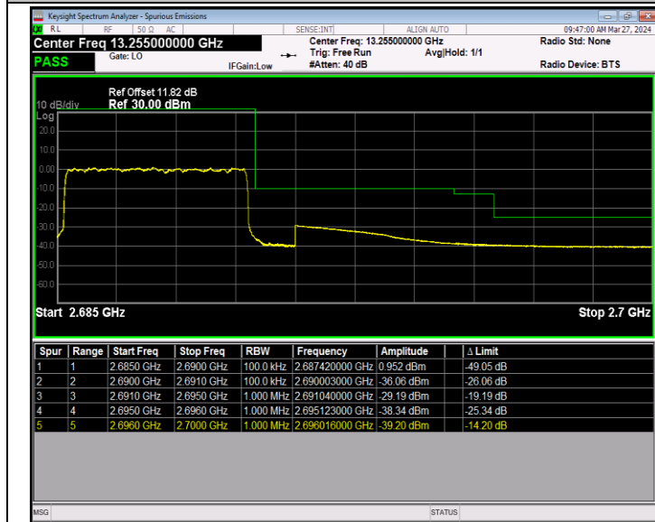
Band41_5MHz_64QAM_41565_25RB#0
