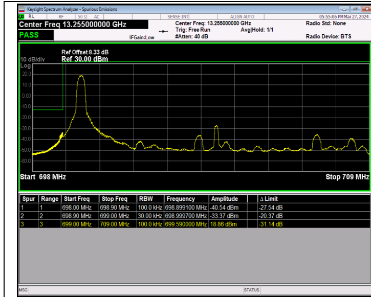
Band12_10MHz_16QAM_23060_1RB#0
