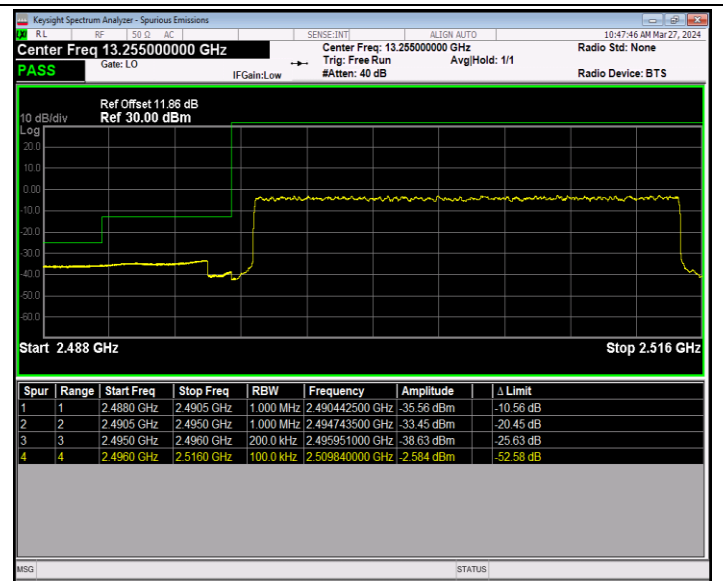
Band41_20MHz_QPSK_39750_100RB#0
