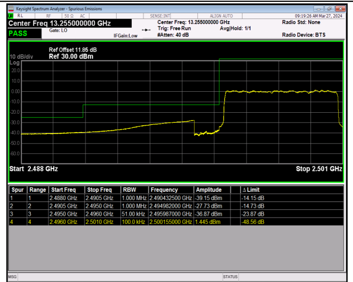
Band41_5MHz_64QAM_39675_25RB#0
