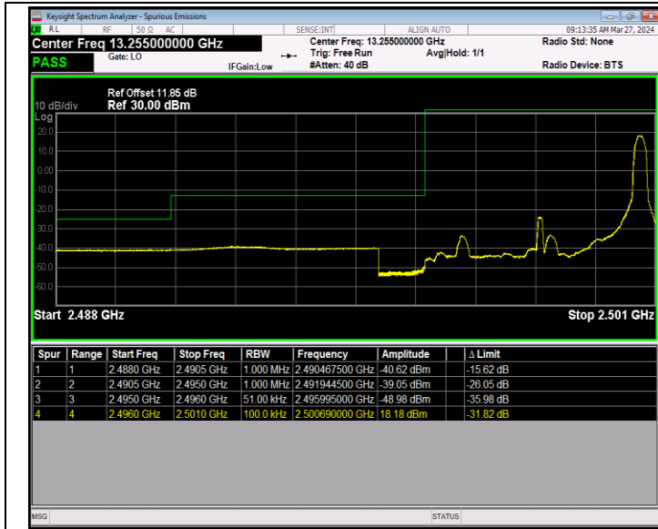
Band41_5MHz_16QAM_39675_1RB#24
