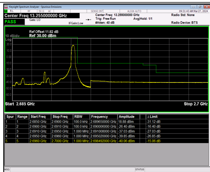
Band41_5MHz_QPSK_41565_1RB#24
