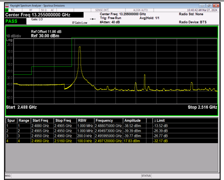
Band41_20MHz_16QAM_39750_1RB#0
