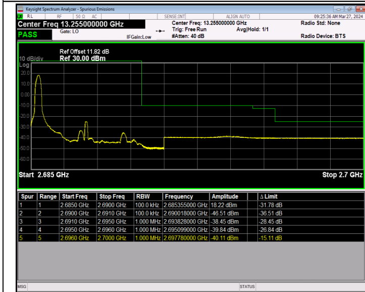
Band41_5MHz_16QAM_41565_1RB#0
