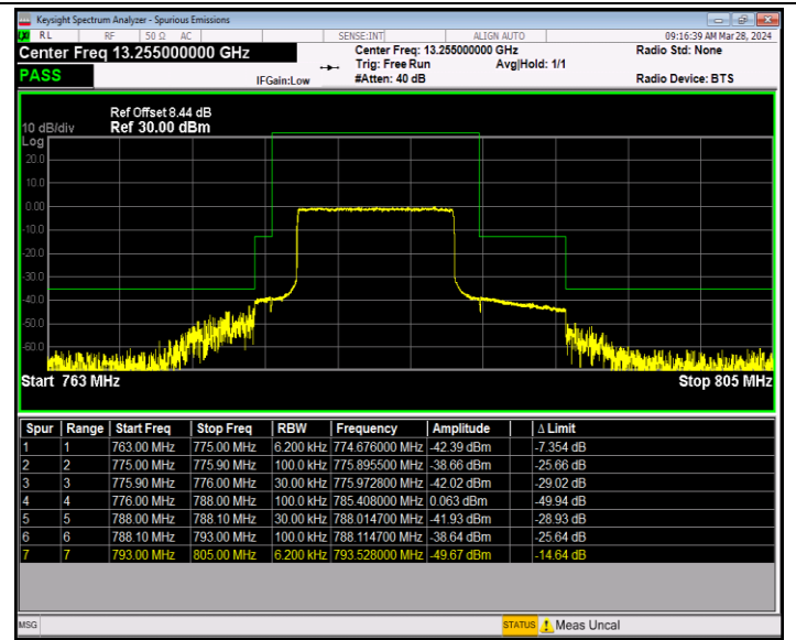
Band13_10MHz_16QAM_23230_50RB#0
