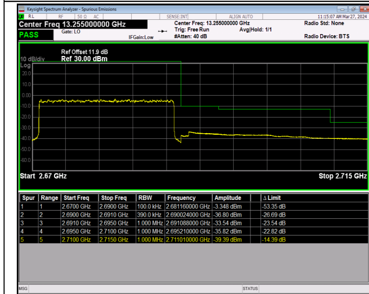
Band41_20MHz_16QAM_41490_100RB#0
