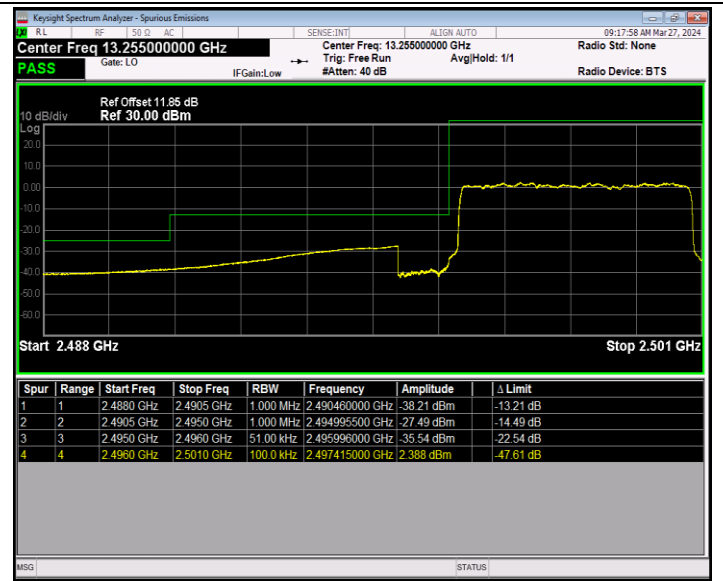
Band41_5MHz_16QAM_39675_25RB#0
