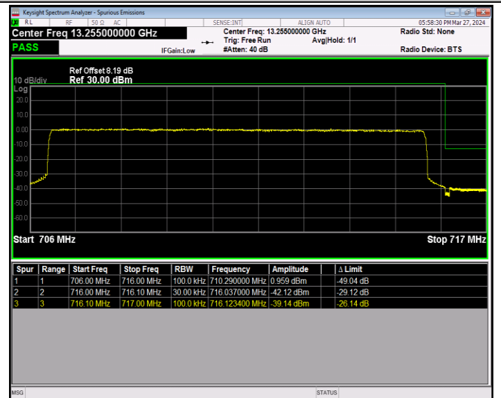
Band12_10MHz_QPSK_23130_50RB#0
