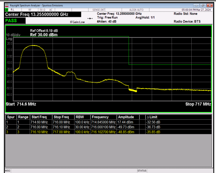
Band12_1.4MHz_64QAM_23173_1RB#0
