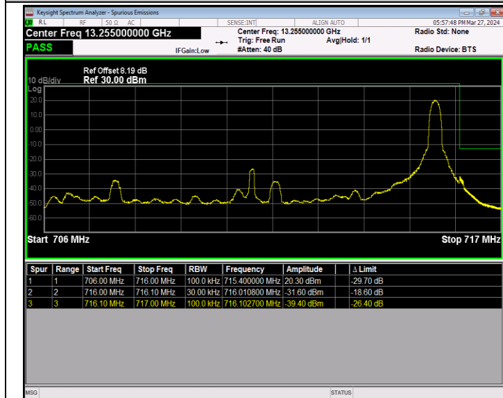
Band12_10MHz_QPSK_23130_1RB#49
