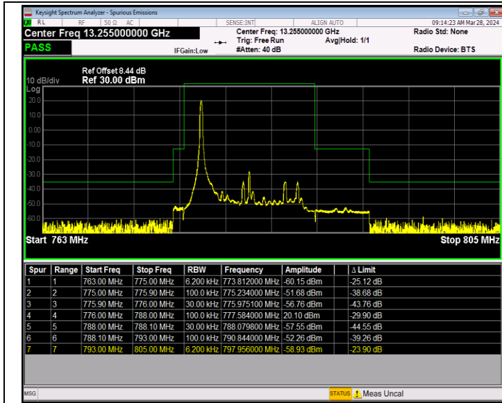
Band13_10MHz_QPSK_23230_1RB#0
