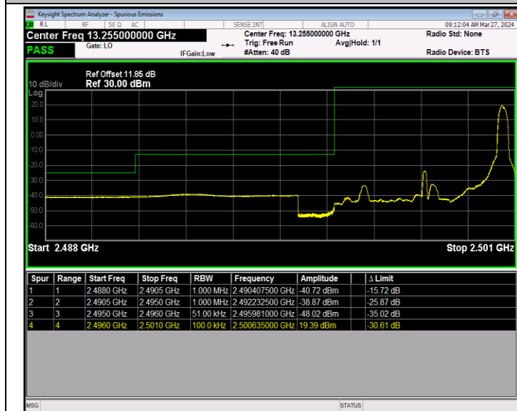
Band41_5MHz_QPSK_39675_1RB#24
