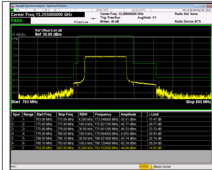
Band13_10MHz_64QAM_23230_50RB#0
