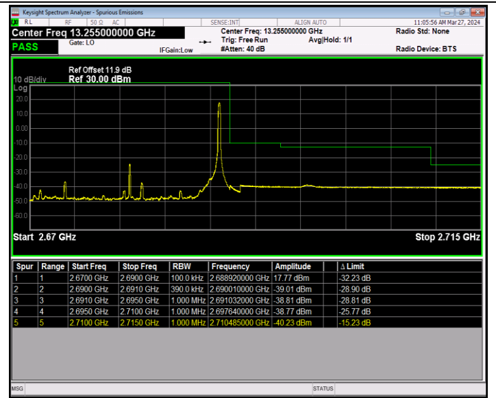
Band41_20MHz_16QAM_41490_1RB#99
