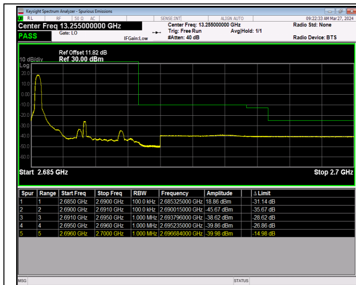
Band41_5MHz_QPSK_41565_1RB#0
