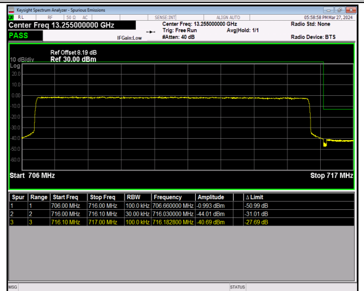
Band12_10MHz_64QAM_23130_50RB#0
