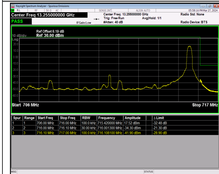
Band12_10MHz_64QAM_23130_1RB#49
