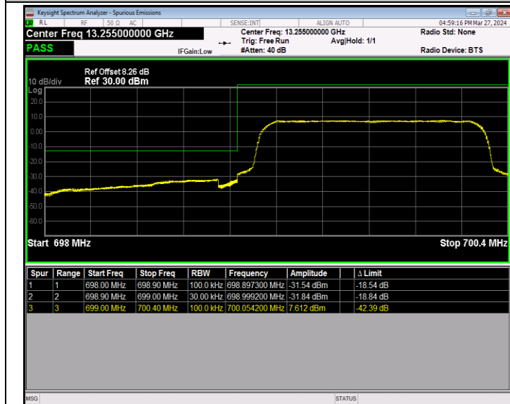
Band12_1.4MHz_64QAM_23017_6RB#0
