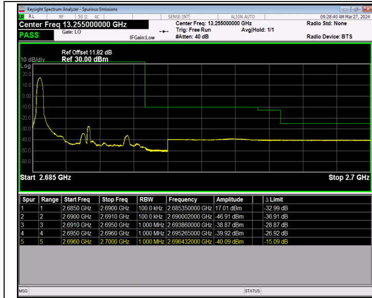
Band41_5MHz_64QAM_41565_1RB#0
