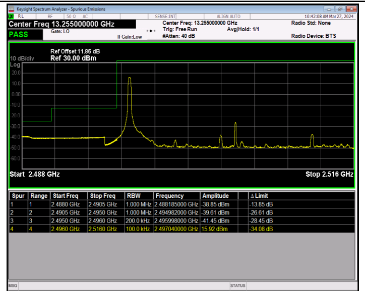
Band41_20MHz_64QAM_39750_1RB#0
