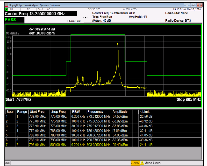
Band13_10MHz_64QAM_23230_1RB#49
