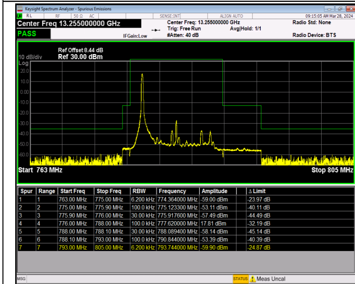
Band13_10MHz_64QAM_23230_1RB#0
