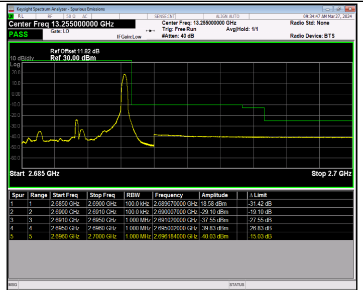
Band41_5MHz_16QAM_41565_1RB#24
