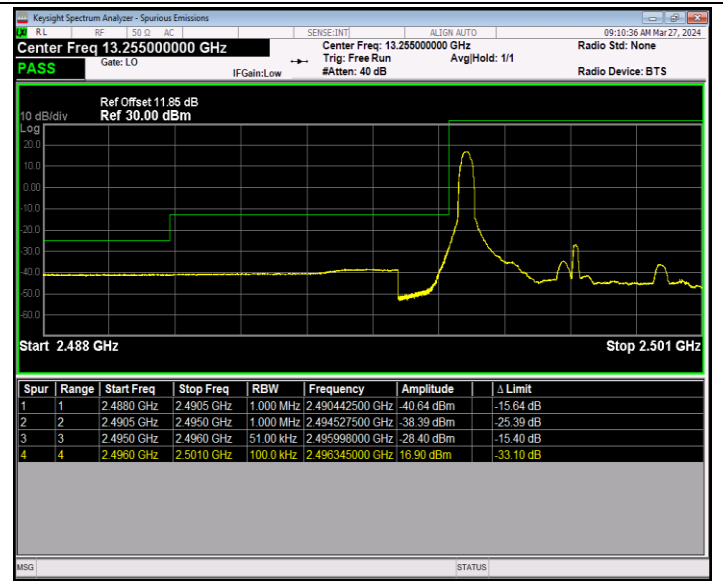
Band41_5MHz_64QAM_39675_1RB#0
