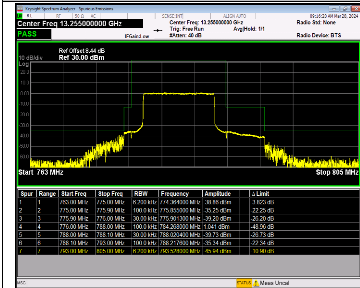
Band13_10MHz_QPSK_23230_50RB#0
