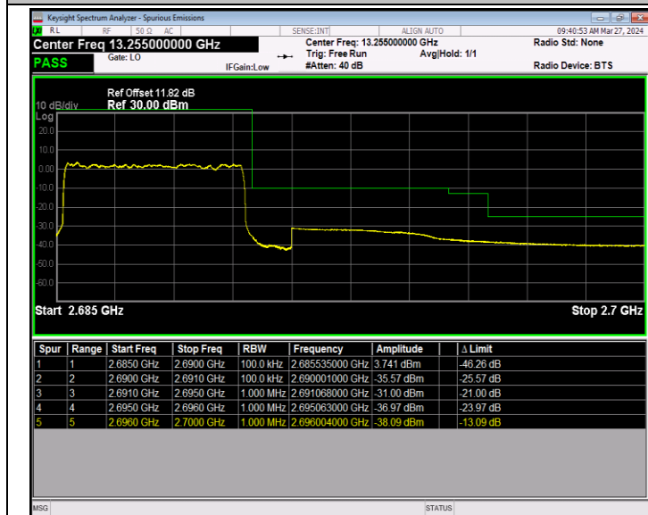
Band41_5MHz_QPSK_41565_25RB#0
