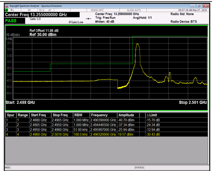
Band41_5MHz_QPSK_39675_1RB#0
