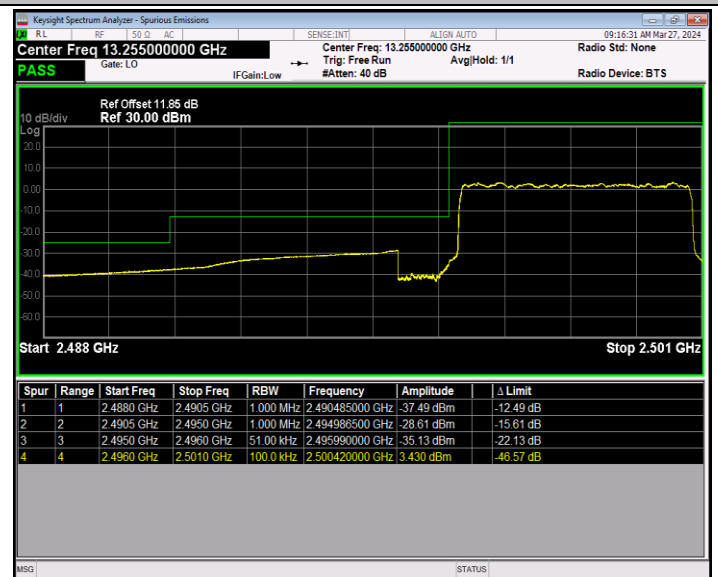
Band41_5MHz_QPSK_39675_25RB#0
