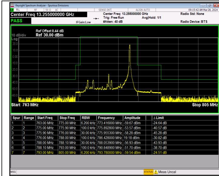
Band13_10MHz_16QAM_23230_1RB#49
