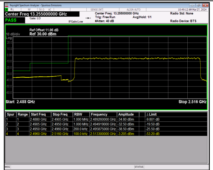
Band41_20MHz_16QAM_39750_100RB#0
