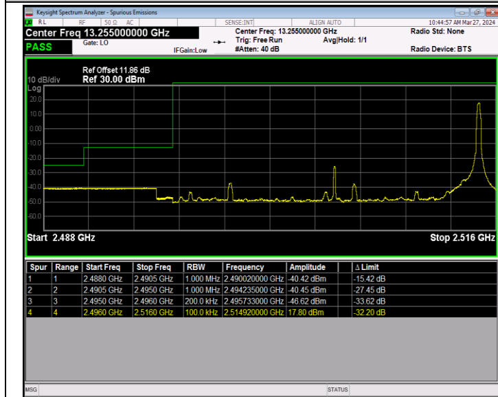
Band41_20MHz_16QAM_39750_1RB#99
