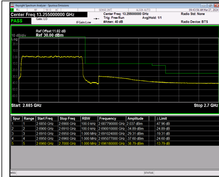
Band41_5MHz_16QAM_41565_25RB#0
