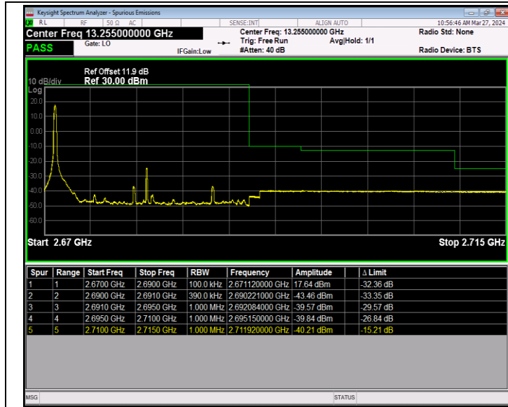
Band41_20MHz_16QAM_41490_1RB#0
