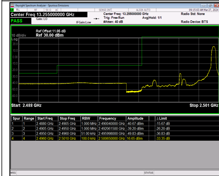
Band41_5MHz_64QAM_39675_1RB#24
