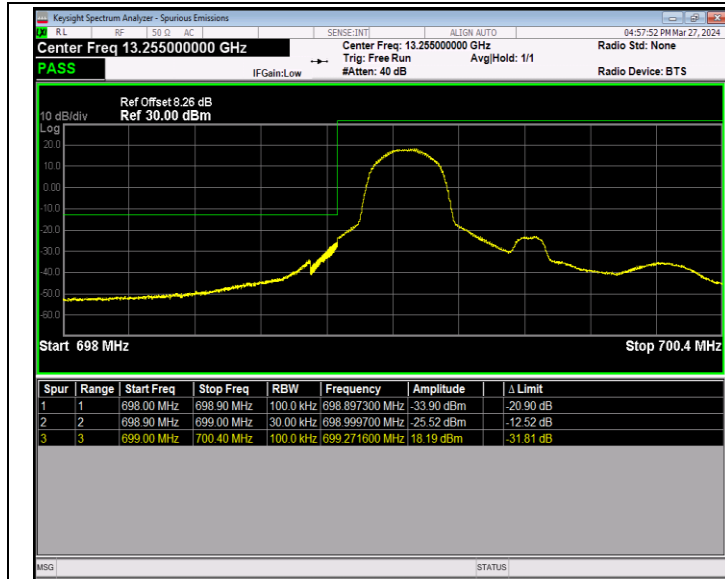
Band12_1.4MHz_64QAM_23017_1RB#0
