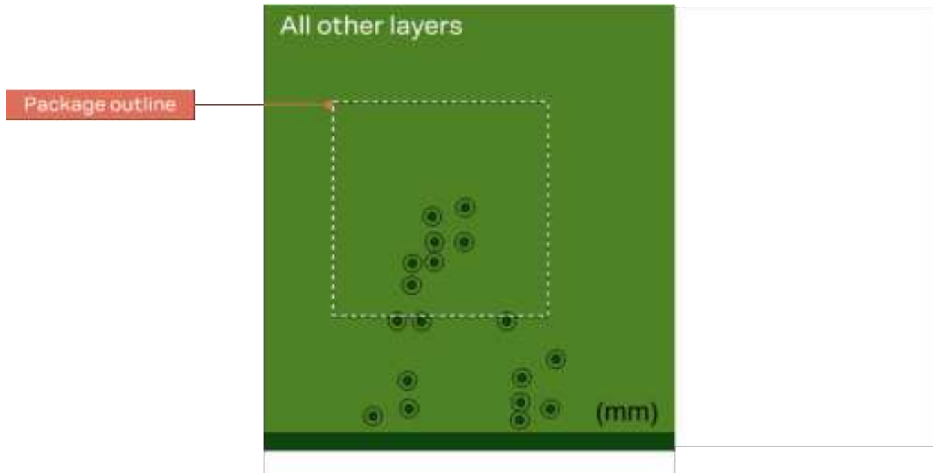
Figure 34: GND layer reference design for external antenna
