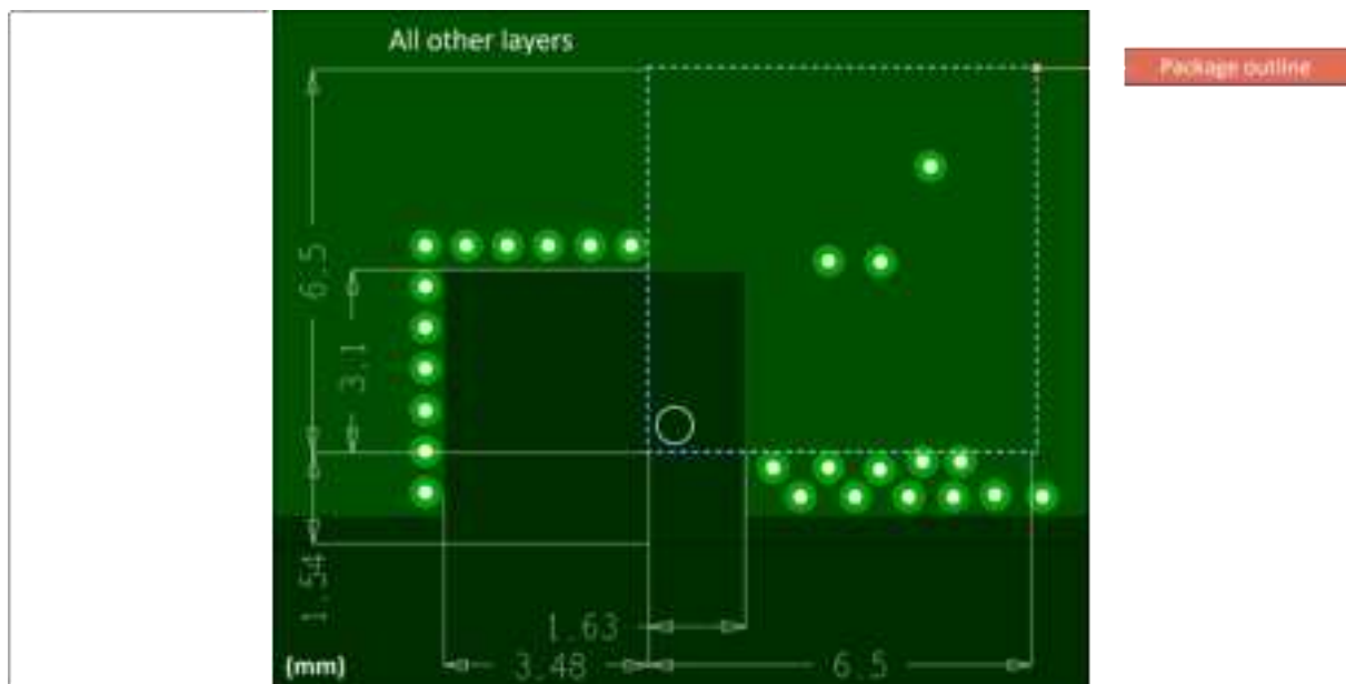
Figure 32: Reference design for internal antenna, edge version, GND layers
