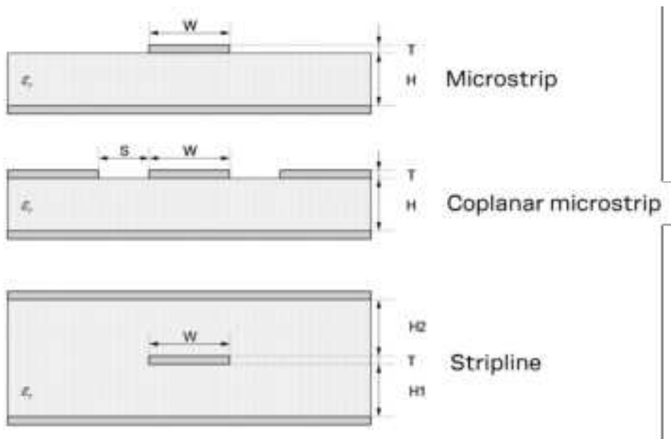
Figure 9: Transmission line trace design
