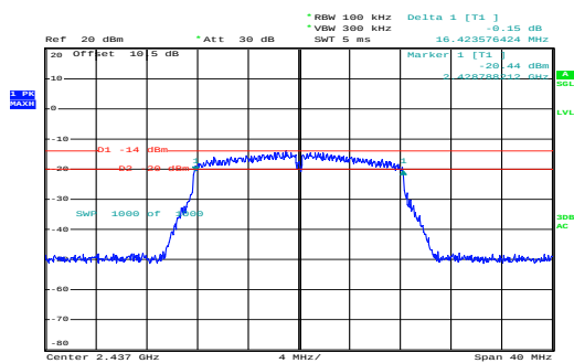
g_2437MHz_Chain 0
