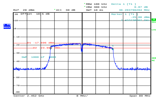
n40_2452MHz_Chain 0
