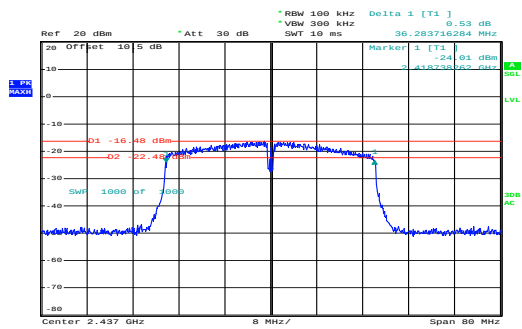
n40_2437MHz_Chain 0
