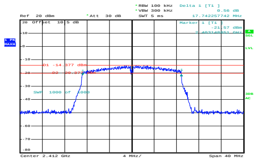
n20_2412MHz_Chain 0
