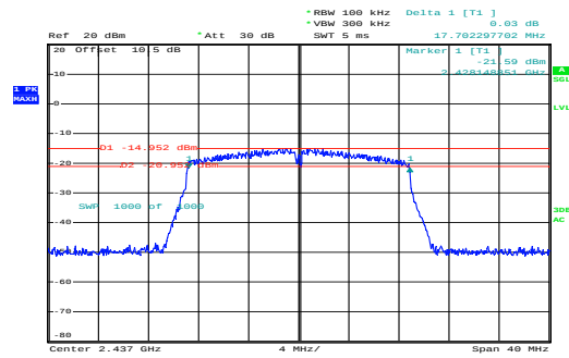
n20_2437MHz_Chain 0
