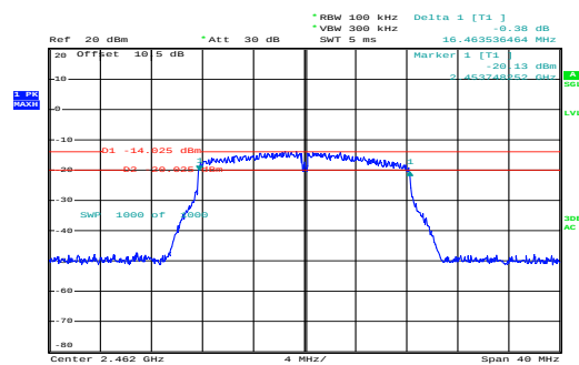
g_2462MHz_Chain 0
