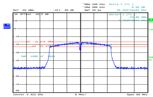
n40_2422MHz_Chain 0
