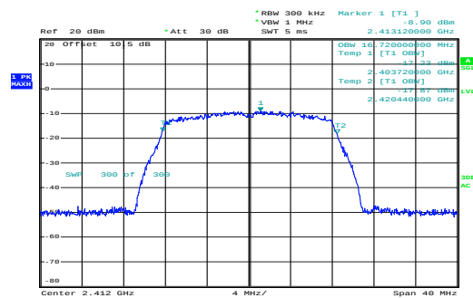
g_2412MHz_Chain 0
