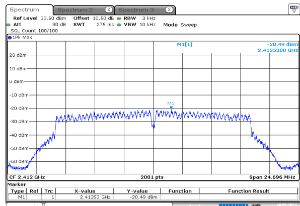
g_2412MHz_Chain 0
