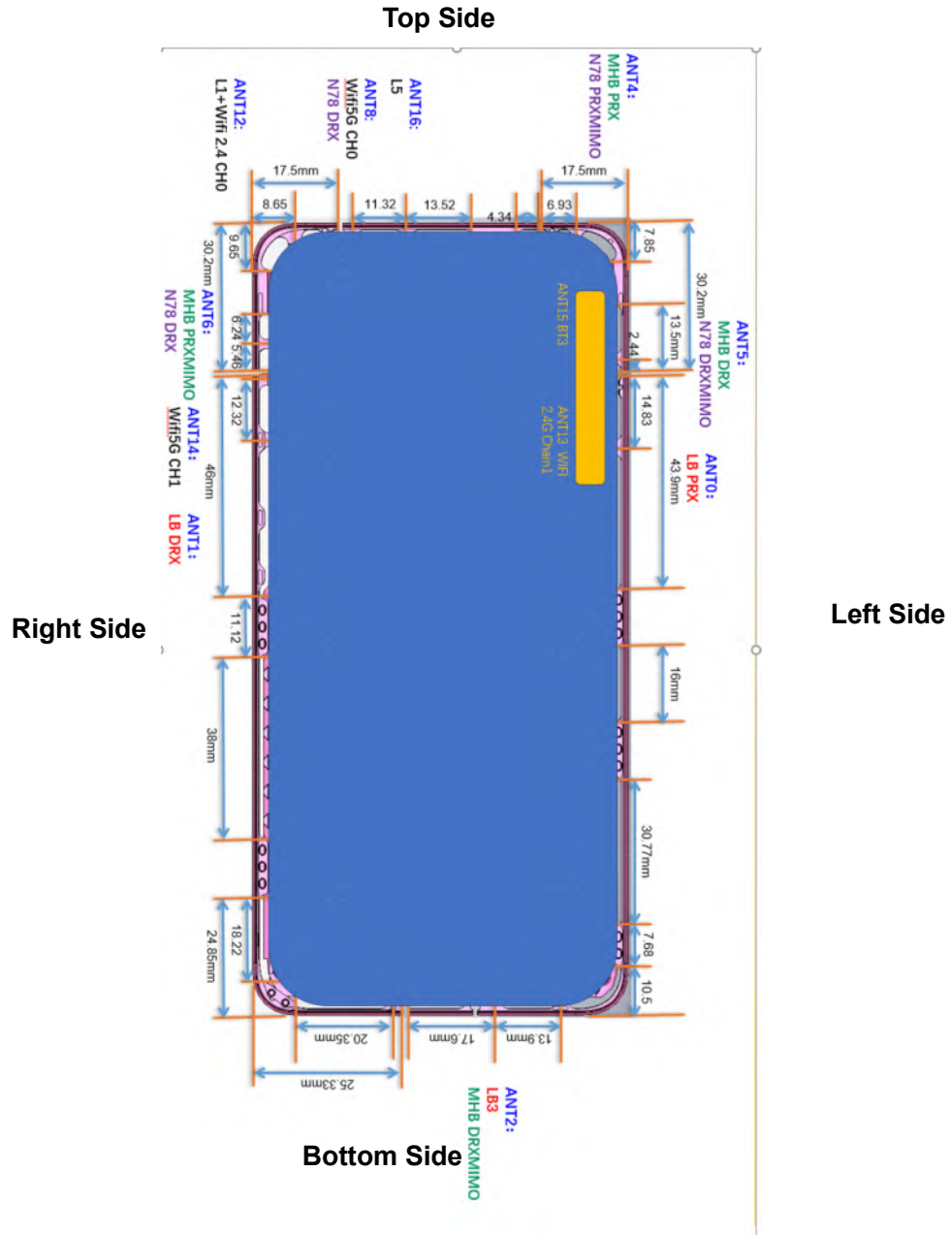
Picture 11.1 Antenna Locations (Back View)
